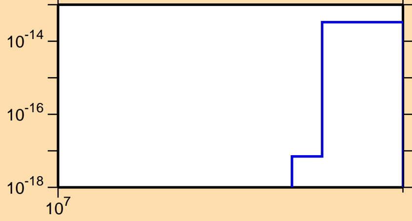
\sigma vs. E for ^{217}\text{Tl} (mt 42)
