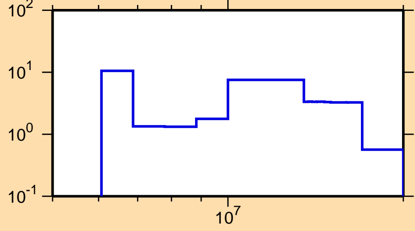
\Delta\sigma/\sigma vs. E for ^{217}\text{Tl}(n,\text{nonel.})
