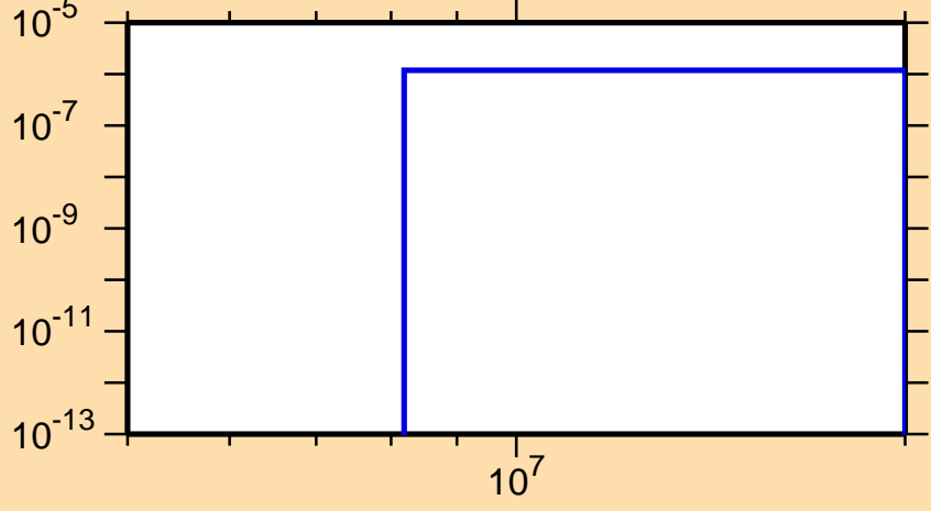
\sigma vs. E for ^{217}\text{Tl}(n,nt)
