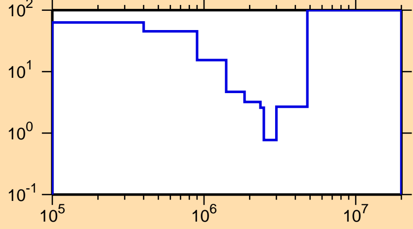
\Delta\sigma/\sigma vs. E for ^{217}\text{Tl}(n,ncont.)
