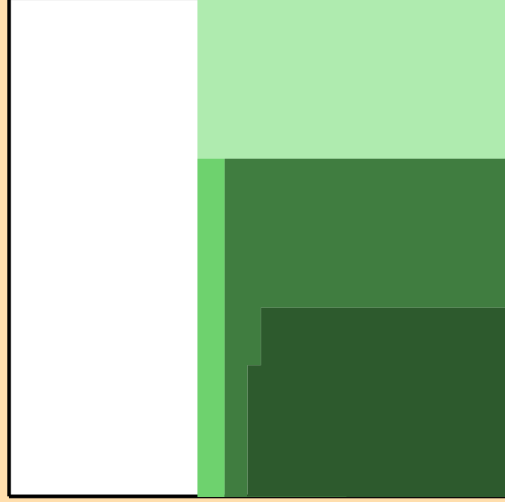
\Delta\sigma/\sigma vs. E for ^{47}\text{V}(n,2n)
