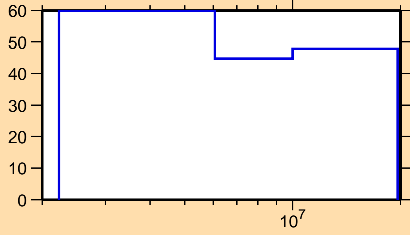
\Delta\sigma/\sigma vs. E for ^{47}\text{V}(n,n\text{cont.})
