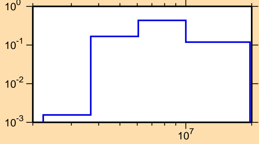
\sigma vs. E for ^{47}\text{V}(n,n\text{cont.})
