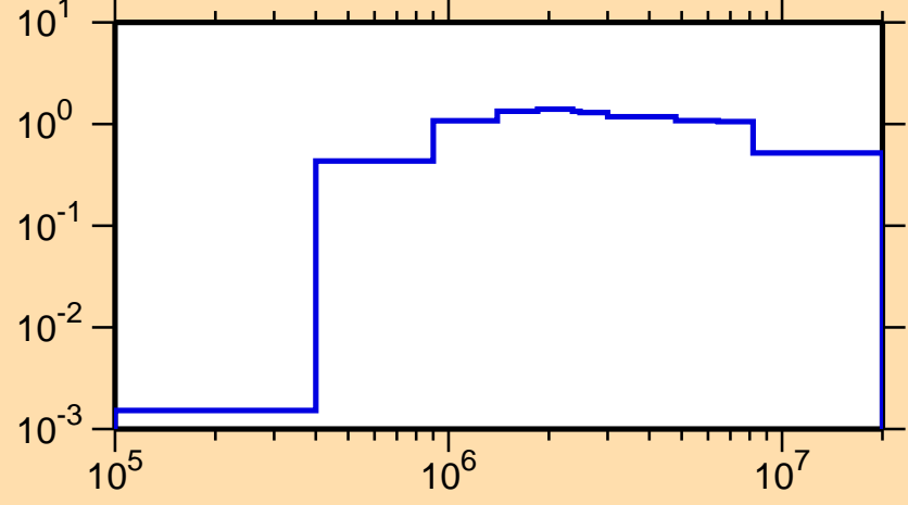
\sigma vs. E for ^{48}\text{V}(n,\text{inel.})
