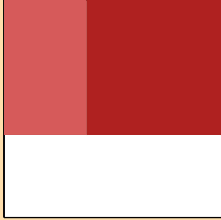
\Delta\sigma/\sigma vs. E for ^{49}\text{V}(n,\text{inel.})
