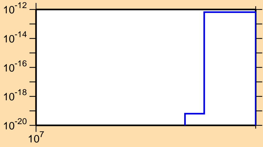
\sigma vs. E for ^{49}\text{V}(\text{mt117})
