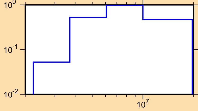
\sigma vs. E for ^{49}\text{V}(n,n\text{cont.})
