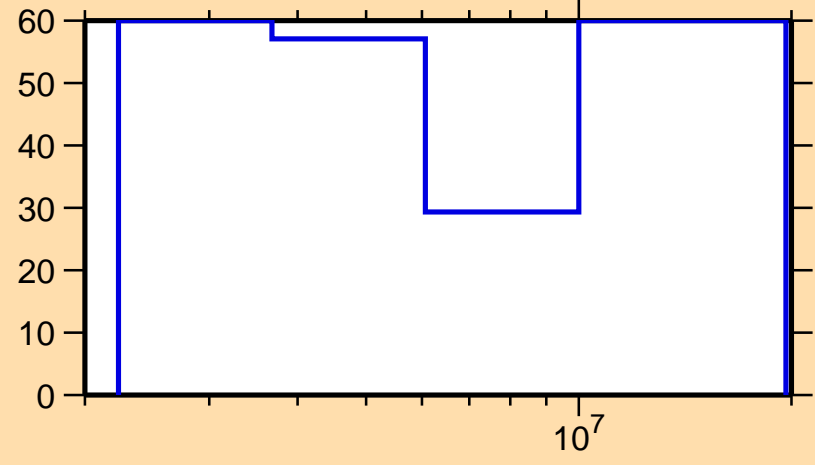
\Delta\sigma/\sigma vs. E for ^{49}\text{V}(n,n\text{cont.})
