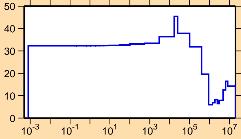
\Delta\sigma/\sigma vs. E for ^{49}\text{V}(n,el.)
