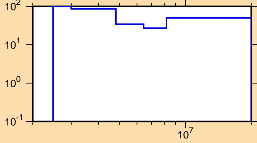
\Delta\sigma/\sigma vs. E for ^{49}\text{V}(n,n\text{cont.})
