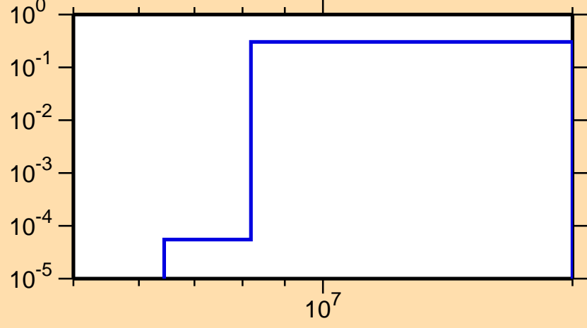
\sigma vs. E for ^{49}\text{V}(n,np)
