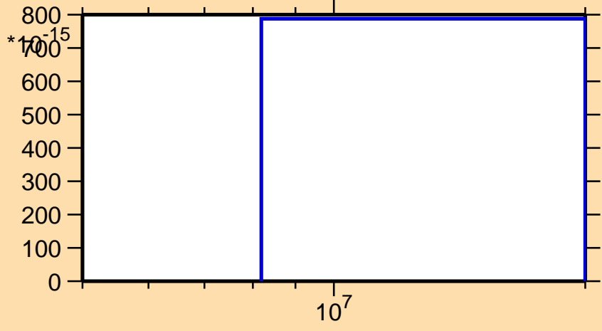
\sigma vs. E for ^{49}\text{V}(n,pd)
