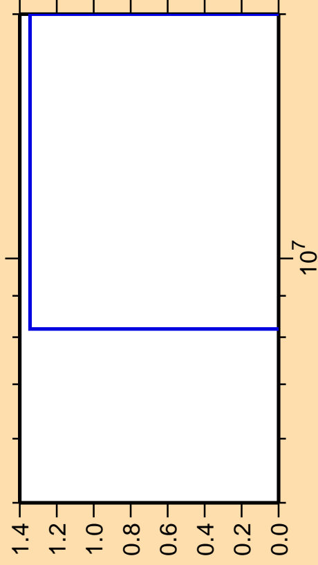
\Delta\sigma/\sigma vs. E for ^{49}\text{V}(n,pd)
