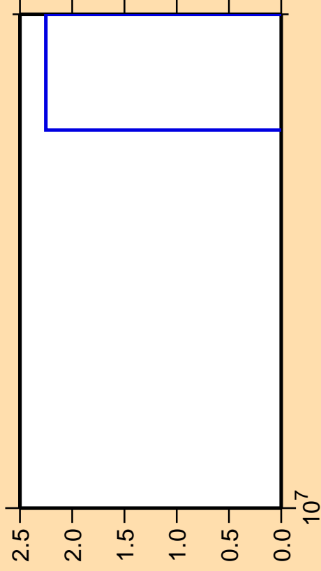
\Delta\sigma/\sigma vs. E for ^{50}\text{V}(n,nt)
