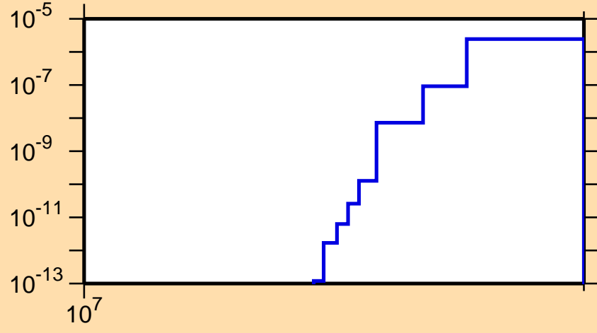
\sigma vs. E for ^{50}\text{V}(n,\text{He}3)
