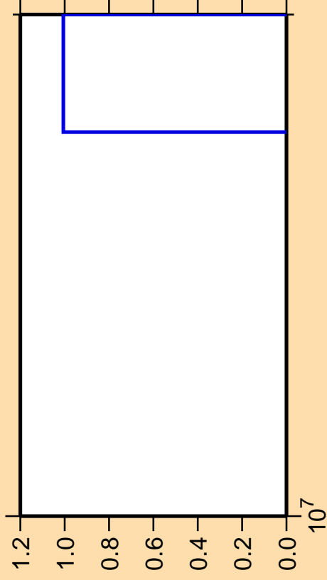
\Delta\sigma/\sigma vs. E for ^{50}\text{V}(n,pd)
