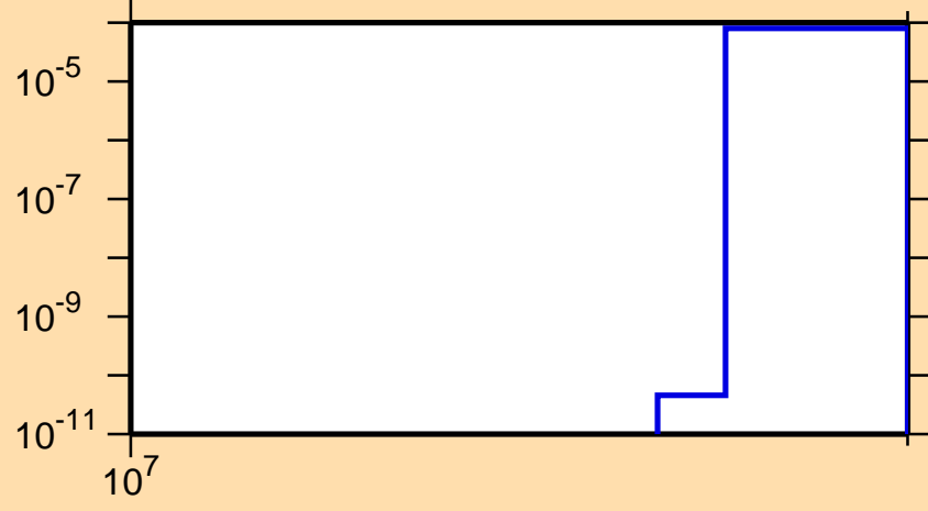
\sigma vs. E for ^{50}\text{V}(n,2np)
