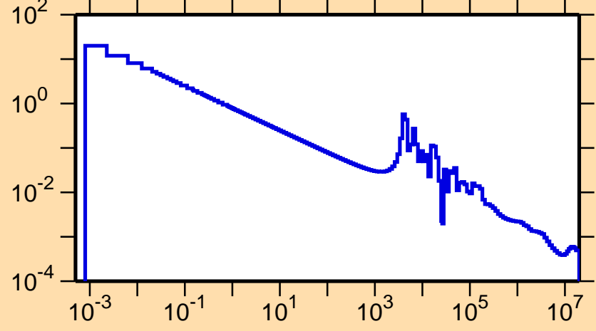
\sigma vs. E for ^{51}\text{V}(n,\gamma)
