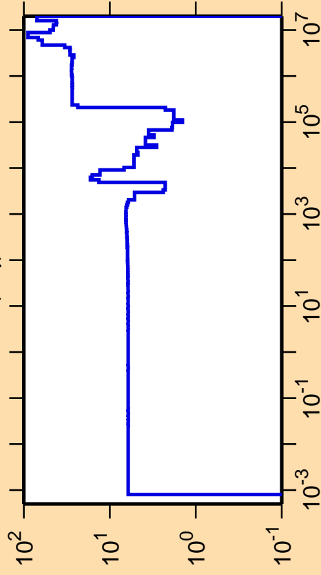
\Delta\sigma/\sigma vs. E for ^{51}\text{V}(n,\gamma)
