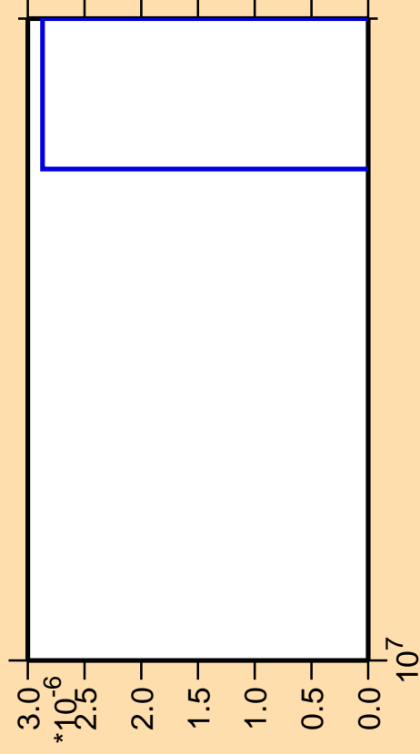
\Delta\sigma/\sigma vs. E for ^{51}\text{V}(n,pd)
