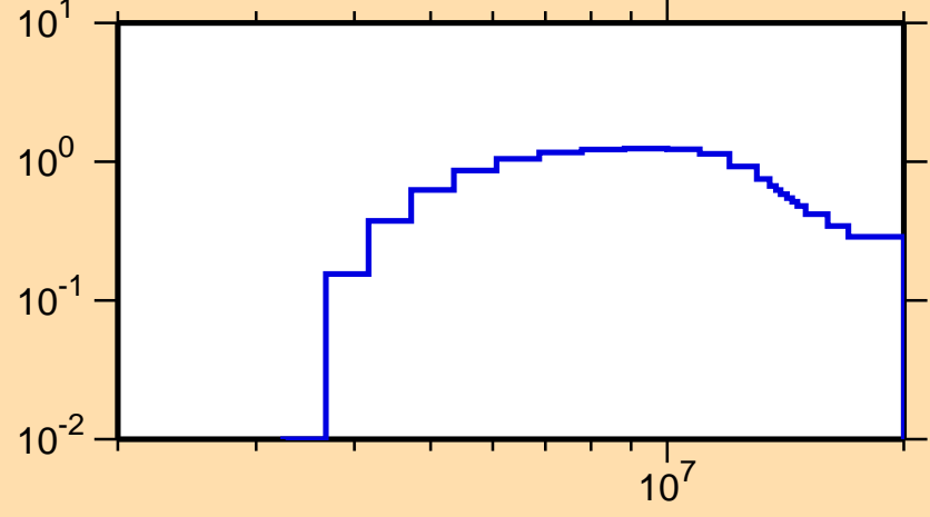
\sigma vs. E for ^{51}\text{V}(n,n\text{cont.})
