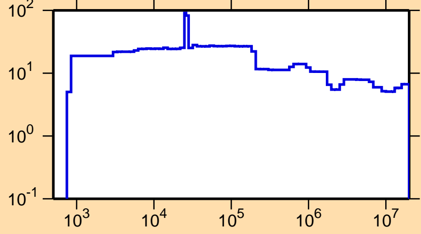
\Delta\sigma/\sigma vs. E for ^{51}\text{V}(n,\text{nonel.})
