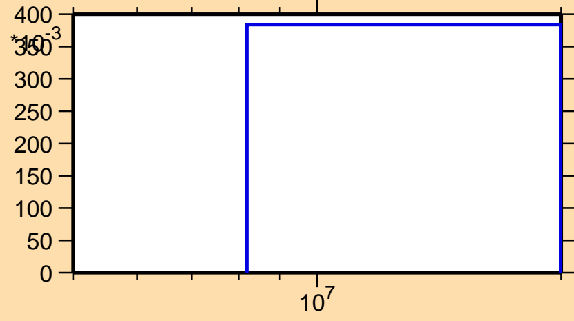
\sigma vs. E for ^{51}\text{V}(n,2n)
