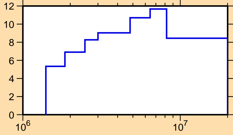
\Delta\sigma/\sigma vs. E for ^{51}\text{V}(n,el.)
