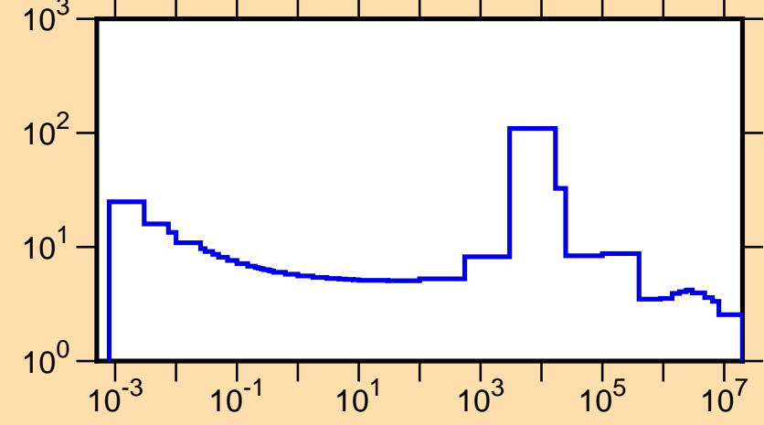
\sigma vs. E for ^{51}\text{V}(n,\text{tot.})
