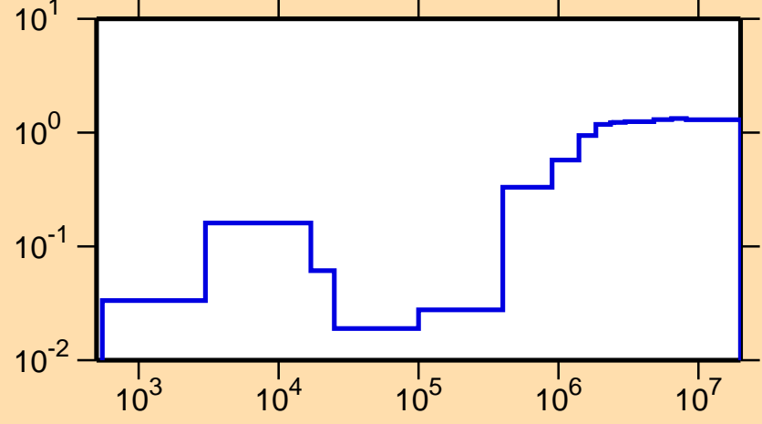
\sigma vs. E for ^{51}\text{V}(n,\text{nonel.})
