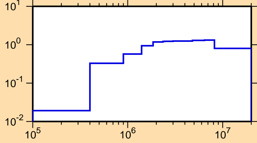
\sigma vs. E for ^{51}\text{V}(n,\text{inel.})
