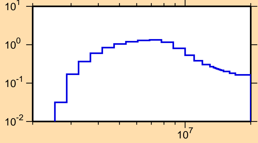
\sigma vs. E for ^{52}\text{V}(n,n\text{cont.})
