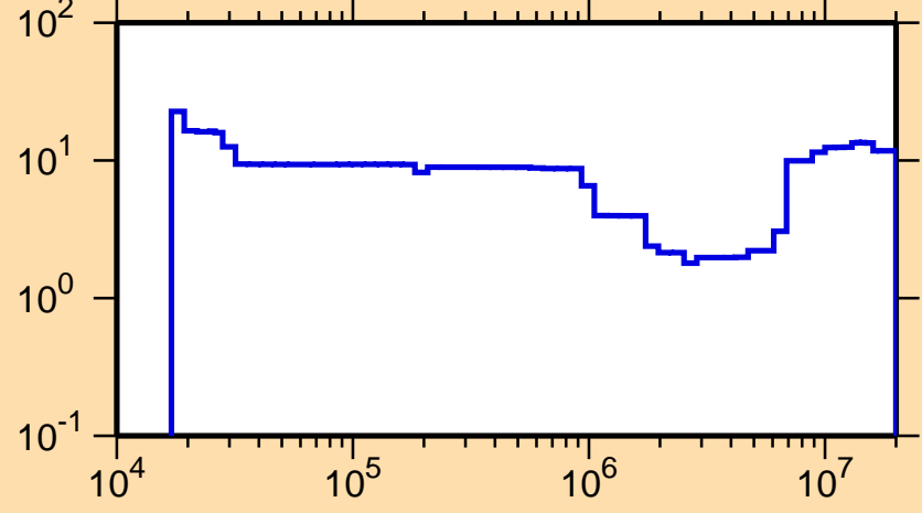
\Delta\sigma/\sigma vs. E for ^{52}\text{V}(n,\text{inel.})
