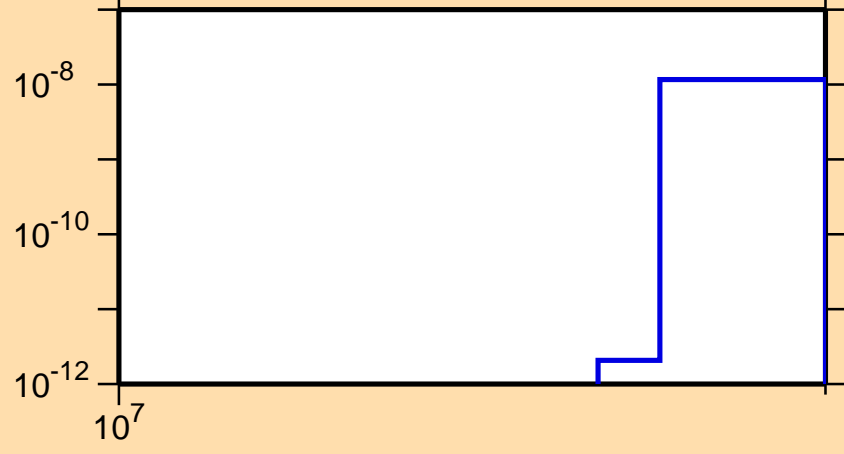
\sigma vs. E for ^{52}\text{V}(n,\text{He}3)
