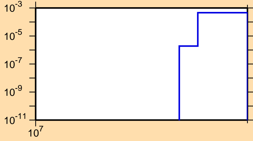
\sigma vs. E for ^{52}\text{V}(n,2np)
