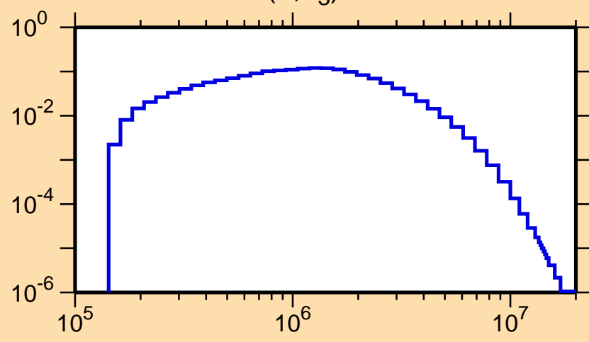
\sigma vs. E for ^{52}\text{V}(n,n_3)
