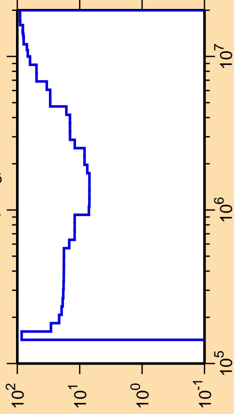
\Delta\sigma/\sigma vs. E for ^{52}\text{V}(n,n_3)
