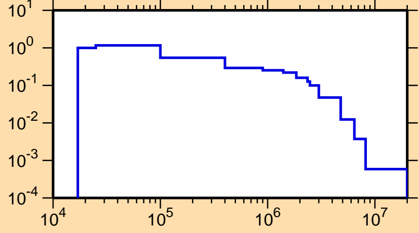
\sigma vs. E for ^{52}\text{V}(n,n_1)
