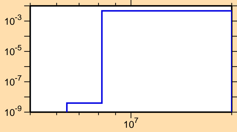
\sigma vs. E for ^{52}\text{V}(n,d)
