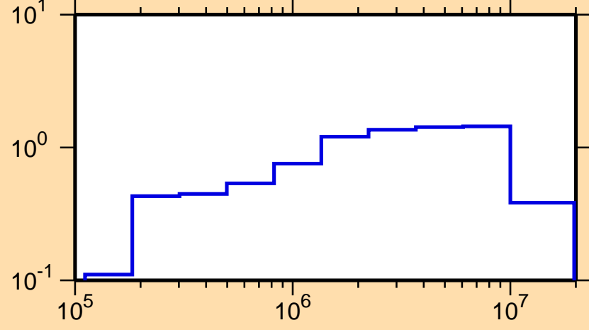
\sigma vs. E for ^{53}\text{V}(n,\text{inel.})
