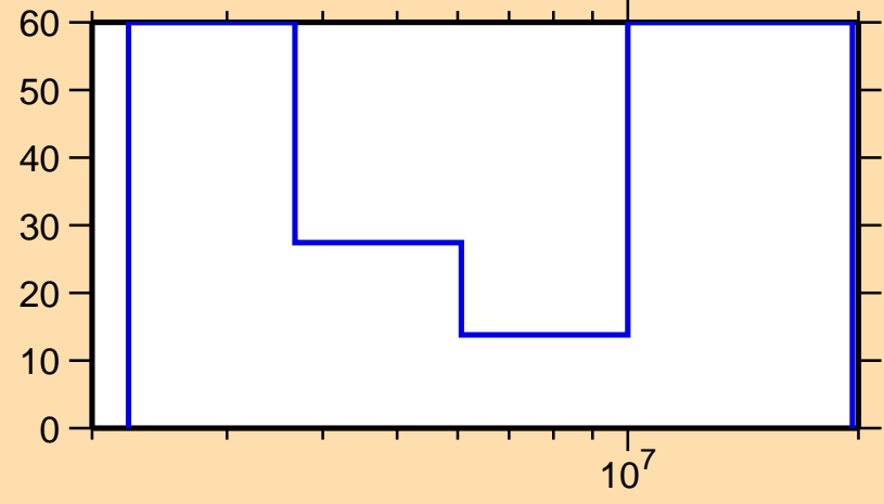
\Delta\sigma/\sigma vs. E for ^{53}\text{V}(n,n\text{cont.})
