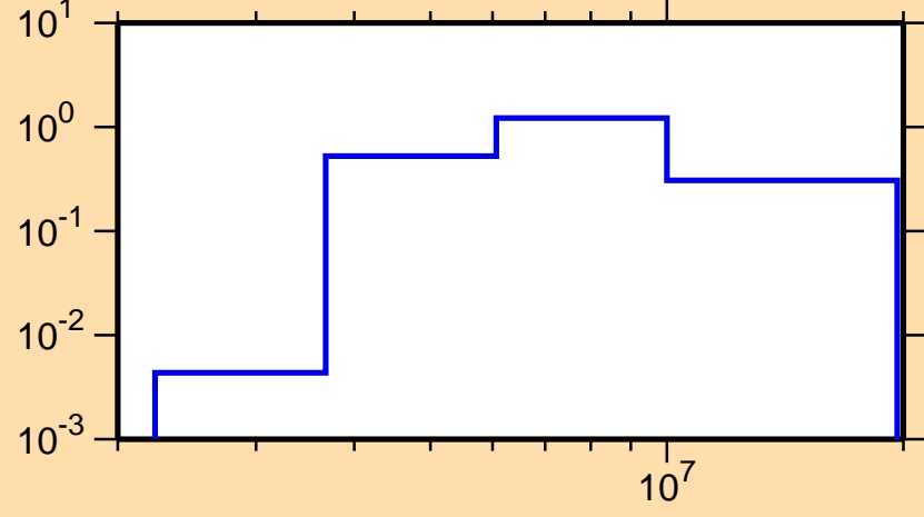
\sigma vs. E for ^{53}\text{V}(n,n\text{cont.})
