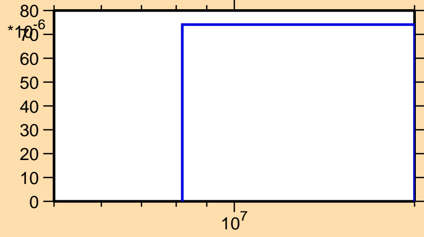
\sigma vs. E for ^{53}\text{V}(n,t)
