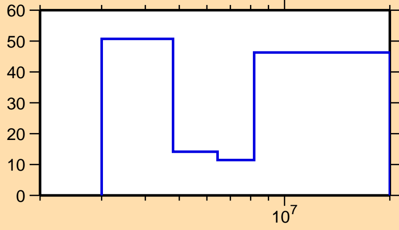
\Delta\sigma/\sigma vs. E for ^{53}\text{V}(n,ncont.)
