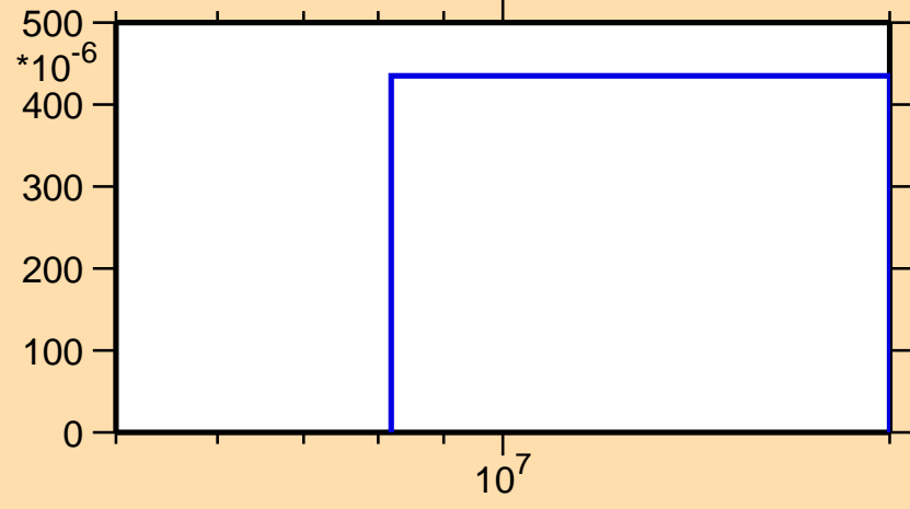
\sigma vs. E for ^{53}\text{V}(n,3n)
