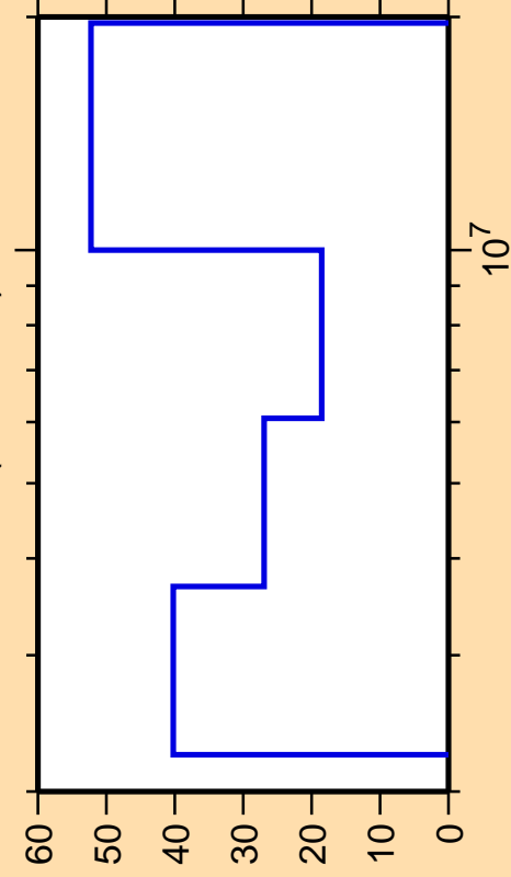
\Delta\sigma/\sigma vs. E for ^{55}\text{V}(n, ncont.)
