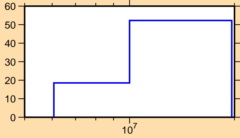
\Delta\sigma/\sigma vs. E for ^{55}\text{V}(n,ncont.)
