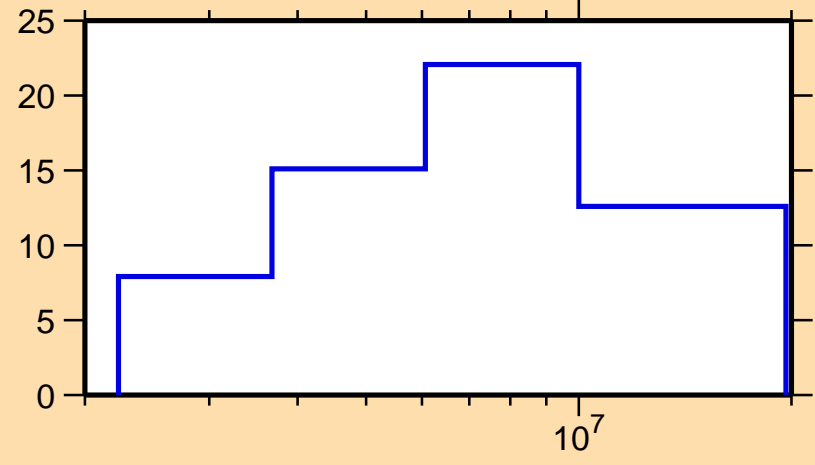
\Delta\sigma/\sigma vs. E for ^{55}\text{V}(n,el.)
