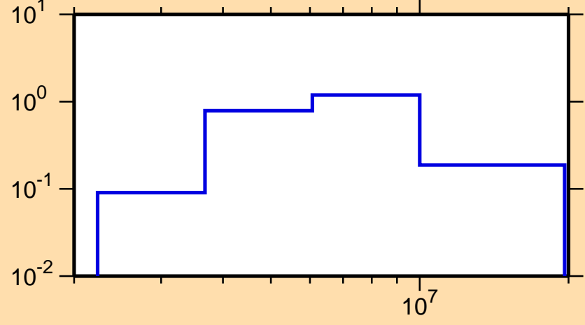
\sigma vs. E for ^{55}\text{V}(n,n\text{cont.})
