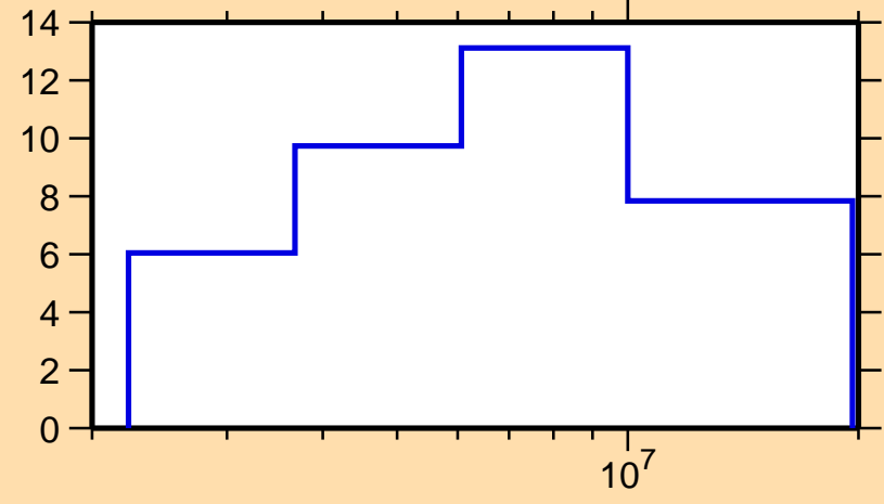
\Delta\sigma/\sigma vs. E for ^{55}\text{V}(n, tot.)
