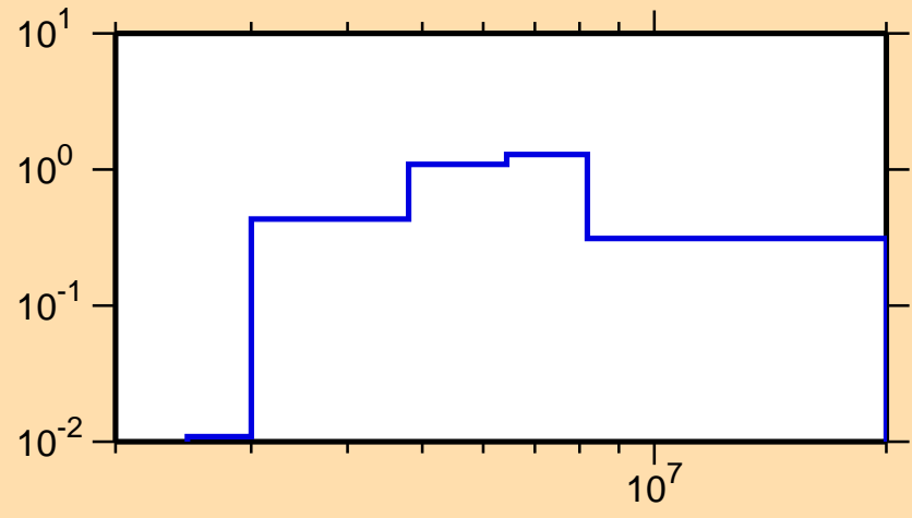
\sigma vs. E for ^{55}\text{V}(n,n\text{cont.})
