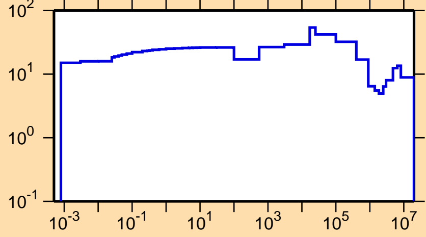
\Delta\sigma/\sigma vs. E for ^{55}\text{V}(n,\text{tot.})
