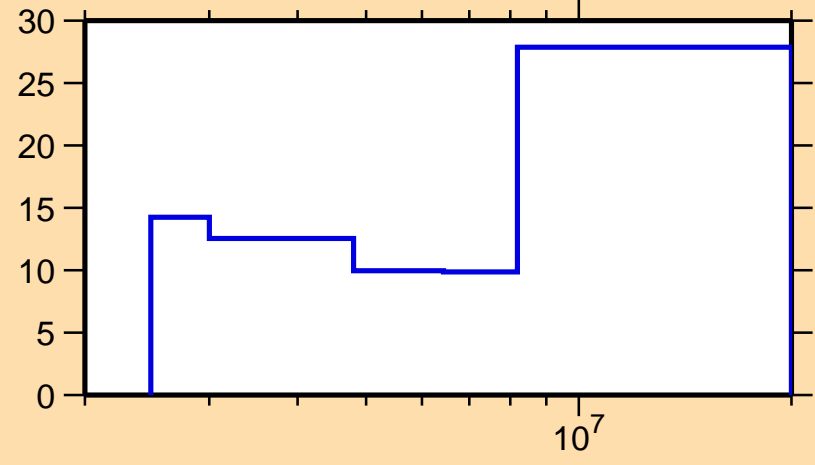
\Delta\sigma/\sigma vs. E for ^{55}\text{V}(n,inel.)
