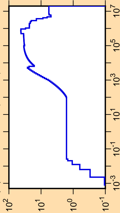
\Delta\mu/\mu vs. E for ^{162}\text{W}(\text{mt251})
