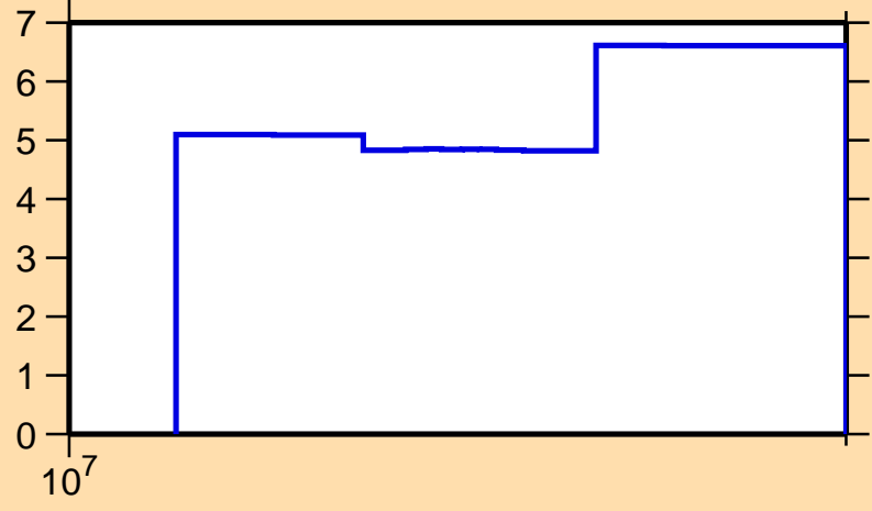
\Delta\sigma/\sigma vs. E for ^{162}\text{W}(n,el.)
