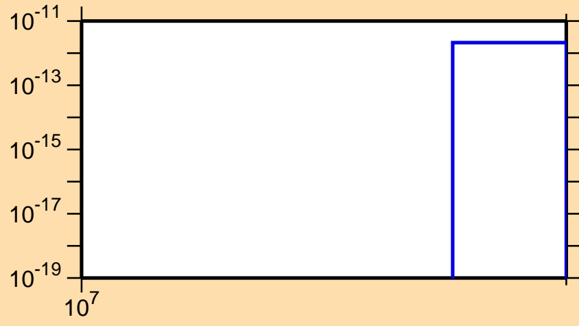
\sigma vs. E for ^{162}\text{W}(n,nt)
