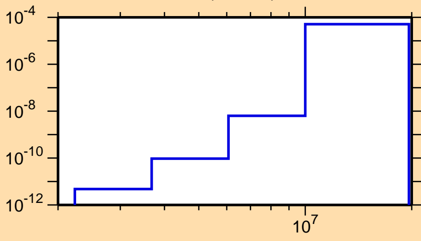
\sigma vs. E for ^{162}\text{W}(n,\text{He}3)
