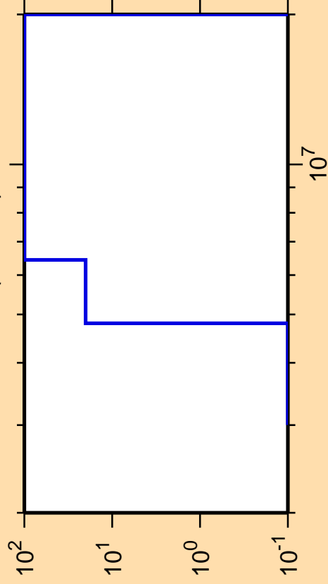
\Delta\sigma/\sigma vs. E for ^{162}\text{W}(\text{mt117})
