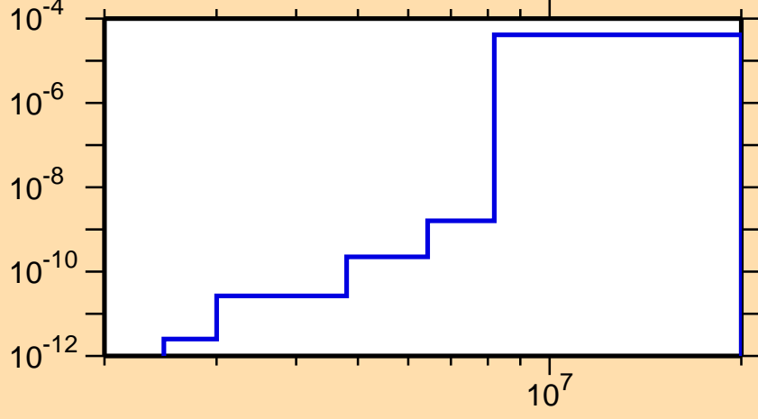
\sigma vs. E for ^{162}\text{W}(n,\text{He}3)
