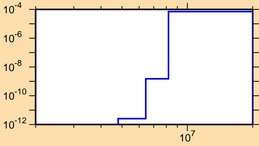
\sigma vs. E for ^{162}\text{W}(\text{mt117})
