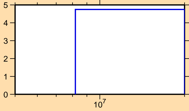
\Delta\sigma/\sigma vs. E for ^{162}\text{W}(n,\text{el.})
