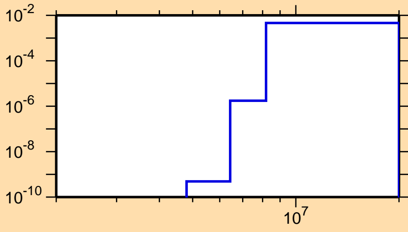
\sigma vs. E for ^{162}\text{W} (mt 45)
