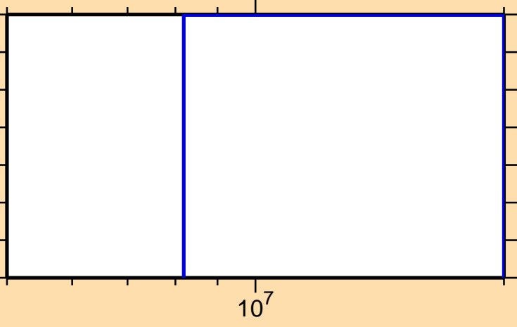
\sigma vs. E for ^{162}\text{W}(n,2n\alpha)
