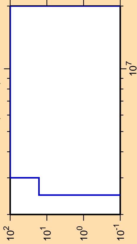
\Delta\sigma/\sigma vs. E for ^{162}\text{W}(n,\text{He}3)
