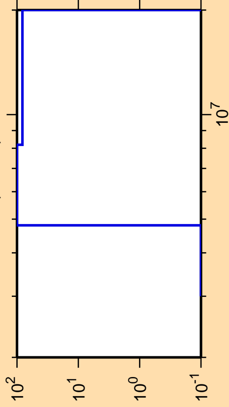
\Delta\sigma/\sigma vs. E for ^{162}\text{W} (mt 45)
