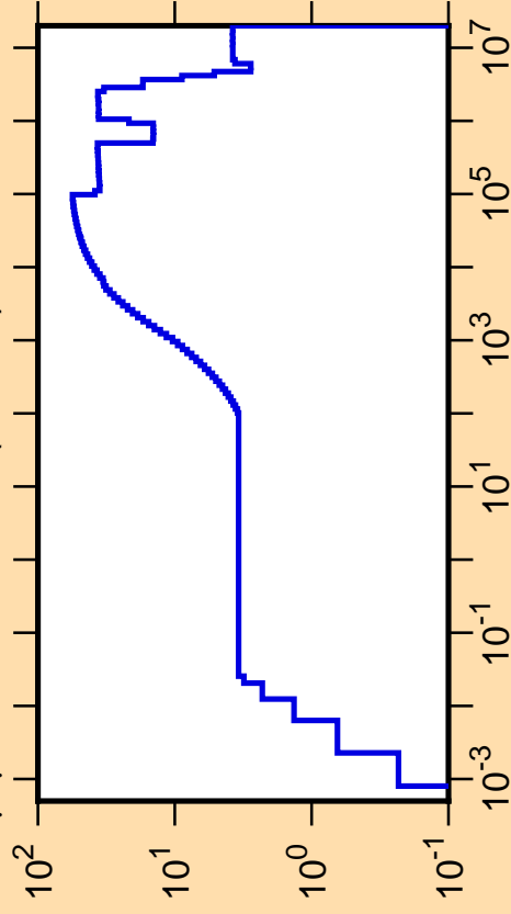
\Delta\mu/\mu vs. E for ^{163}\text{W}(\text{mt251})
