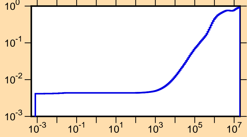
\mu vs. E for ^{163}\text{W}(\text{mt251})
