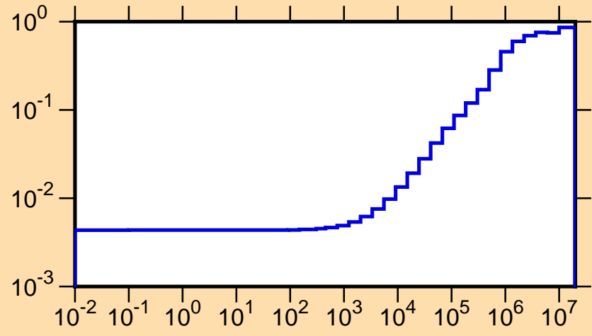
\mu vs. E for ^{163}\text{W}(\text{mt251})
