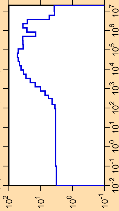
\Delta\mu/\mu vs. E for ^{163}\text{W}(\text{mt251})
