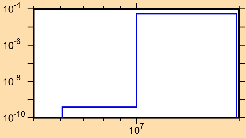
\sigma vs. E for ^{163}\text{W} (mt 45)
