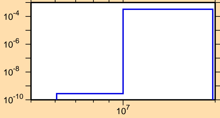
\sigma vs. E for ^{163}\text{W}(n,t)
