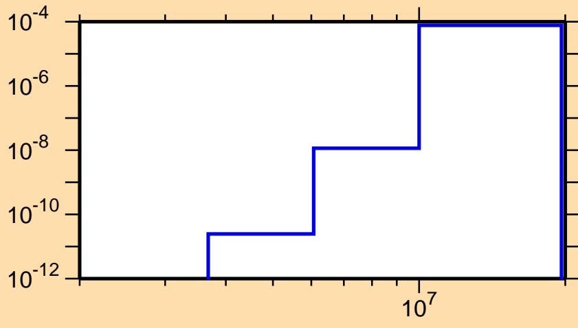
\sigma vs. E for ^{163}\text{W}(n,\text{He}3)
