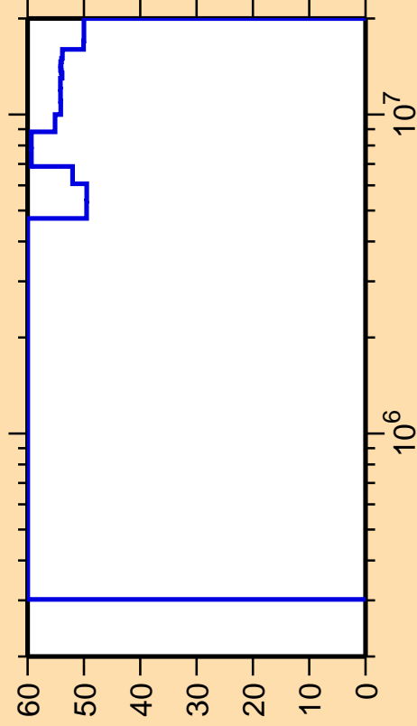
\Delta\sigma/\sigma vs. E for ^{164}\text{W}(n,\text{inel.})
