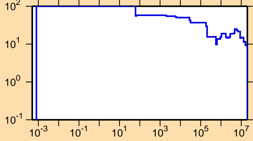
\Delta\sigma/\sigma vs. E for ^{164}\text{W}(n,\text{el.})
