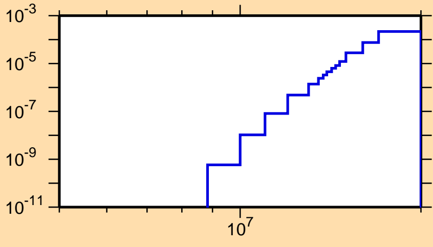
\sigma vs. E for ^{164}\text{W} (mt 45)
