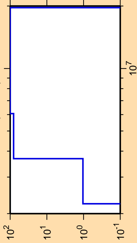
\Delta\sigma/\sigma vs. E for ^{164}\text{W}(n,\text{He}3)
