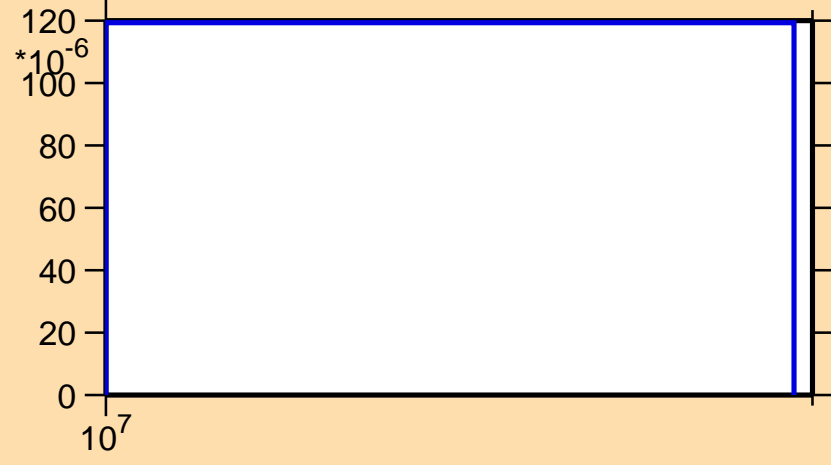
\sigma vs. E for ^{164}\text{W}(n,2n\alpha)
