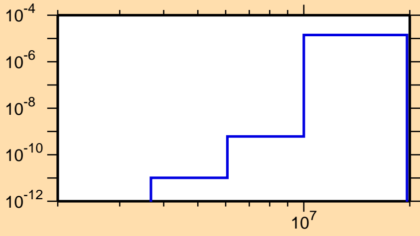
\sigma vs. E for ^{164}\text{W}(n,\text{He}3)
