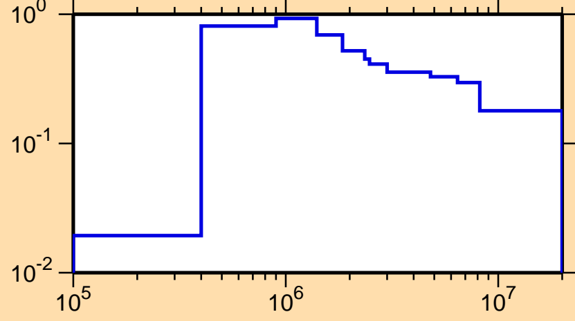
\sigma vs. E for ^{164}\text{W}(n,\text{inel.})
