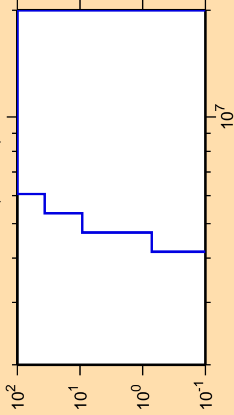
\Delta\sigma/\sigma vs. E for ^{165}\text{W}(n,\text{He}3)
