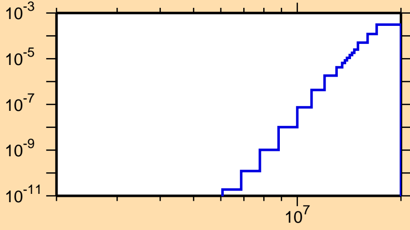
\sigma vs. E for ^{165}\text{W}(n,\text{He}3)
