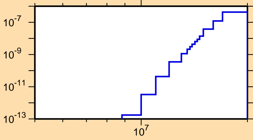
\sigma vs. E for ^{165}\text{W}(\text{mt117})
