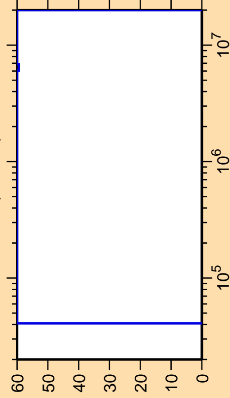
\Delta\sigma/\sigma vs. E for ^{165}\text{W}(n,\text{inel.})
