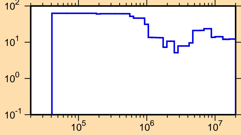
\Delta\sigma/\sigma vs. E for ^{165}\text{W}(n,\text{tot.})
