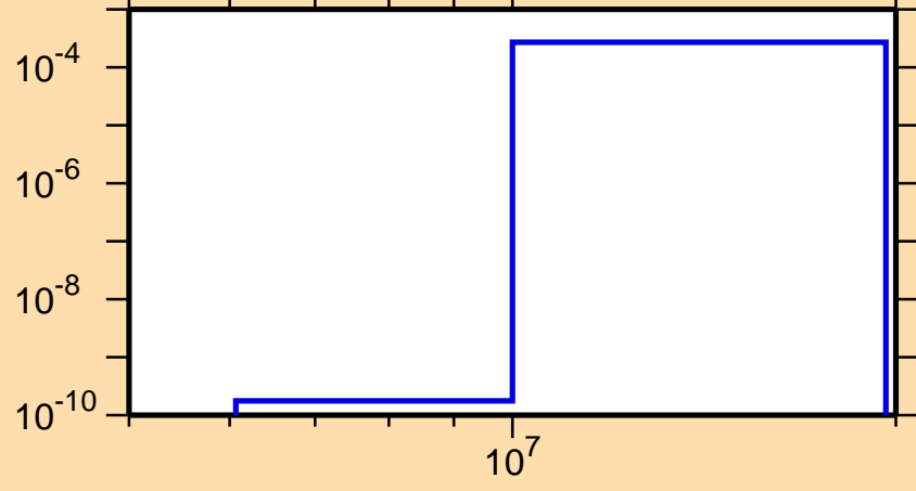
\sigma vs. E for ^{165}\text{W}(n,t)
