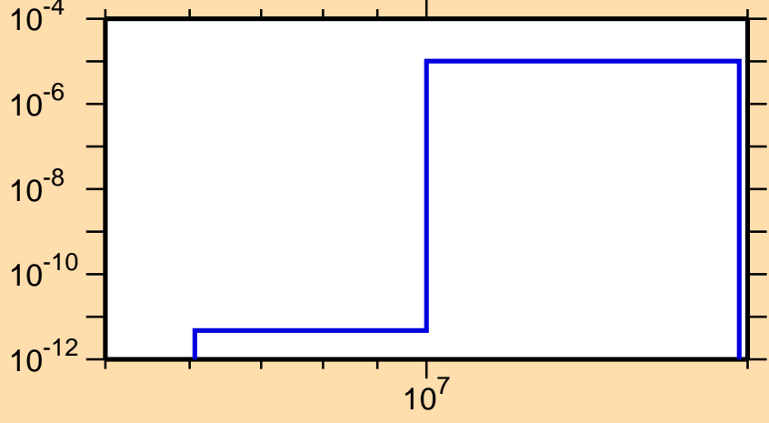
\sigma vs. E for ^{165}\text{W} (mt 45)
