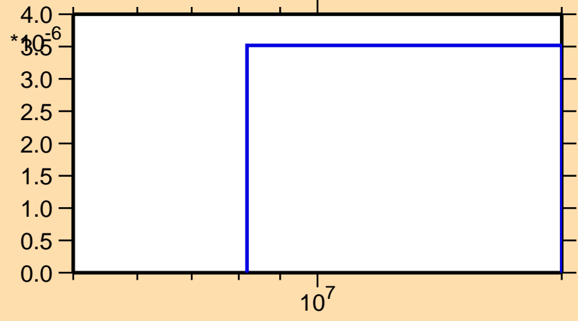
\sigma vs. E for ^{165}\text{W}(n,\text{pd})
