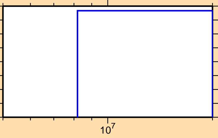
\sigma vs. E for ^{165}\text{W}(\text{mt117})
