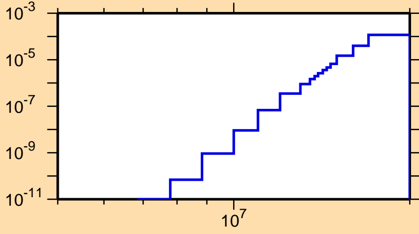
\sigma vs. E for ^{167}\text{W}(n,\text{He}3)
