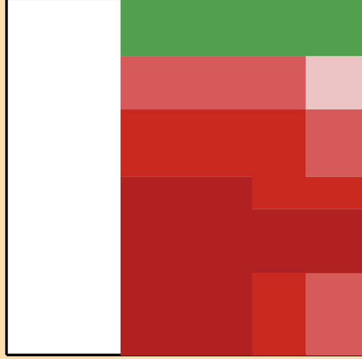
\Delta\sigma/\sigma vs. E for ^{167}\text{W}(n,2n)
