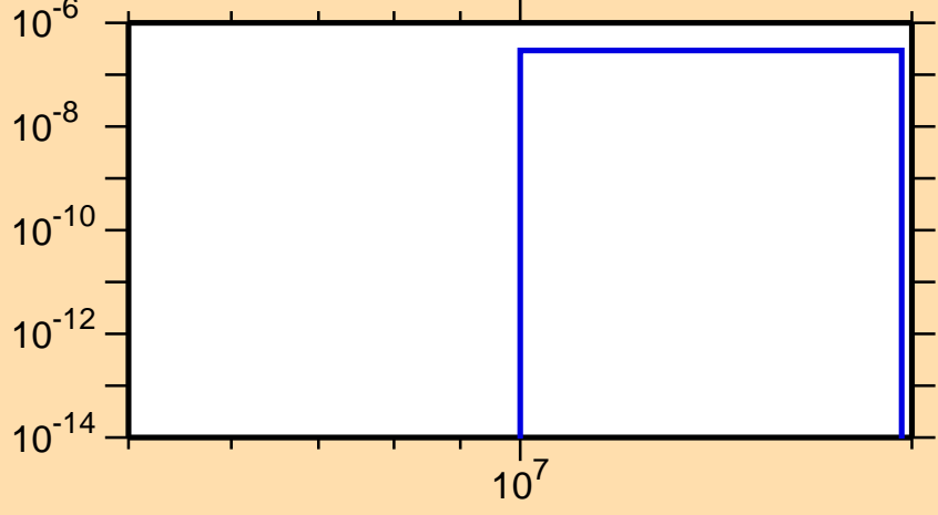
\sigma vs. E for ^{167}\text{W}(n,\text{nd})
