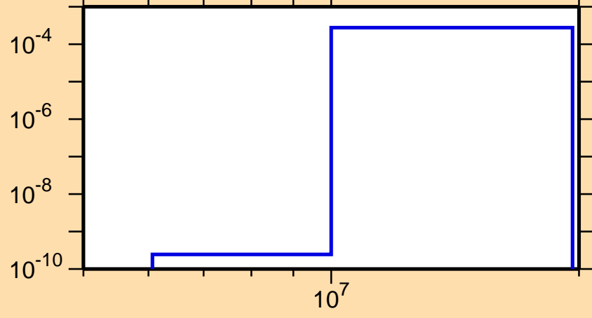
\sigma vs. E for ^{167}\text{W}(n,t)
