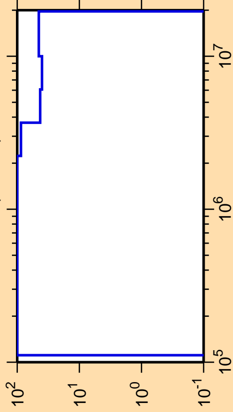
\Delta\sigma/\sigma vs. E for ^{167}\text{W}(n,\text{inel.})
