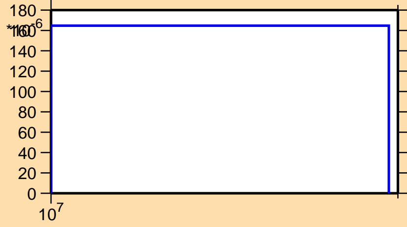
\sigma vs. E for ^{167}\text{W}(n,2np)
