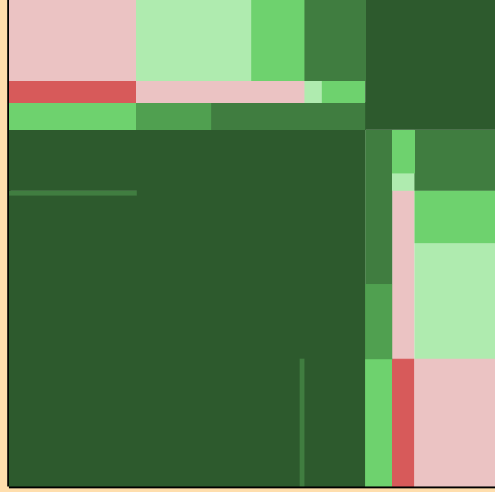
\sigma vs. E for ^{167}\text{W}(n,\text{inel.})
