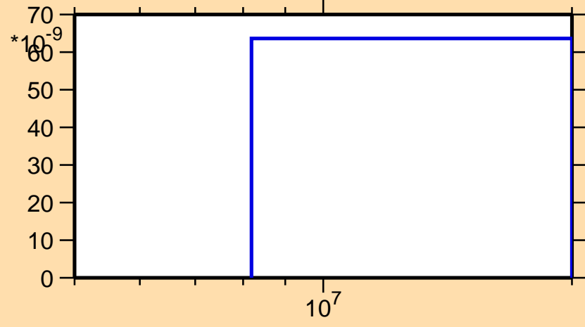
\sigma vs. E for ^{167}\text{W}(n,\text{pt})
