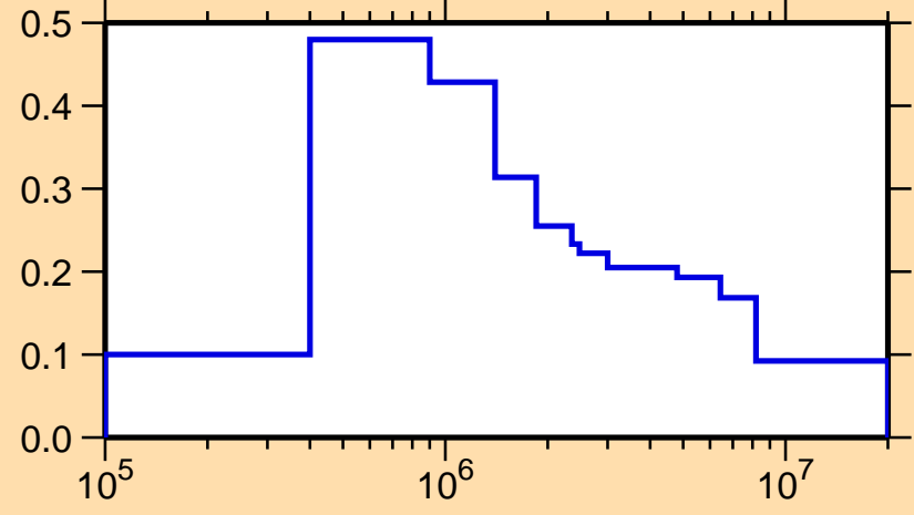
\sigma vs. E for ^{167}\text{W}(n,n_1)
