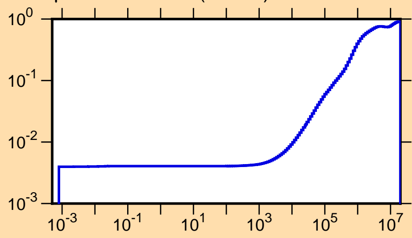
\mu vs. E for ^{170}\text{W}(\text{mt251})
