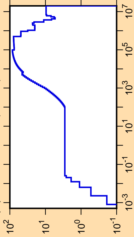
\Delta\mu/\mu vs. E for ^{170}\text{W}(\text{mt251})
