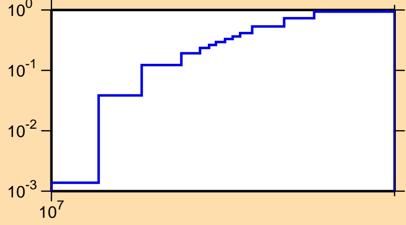
\sigma vs. E for ^{170}\text{W}(n,2n)
