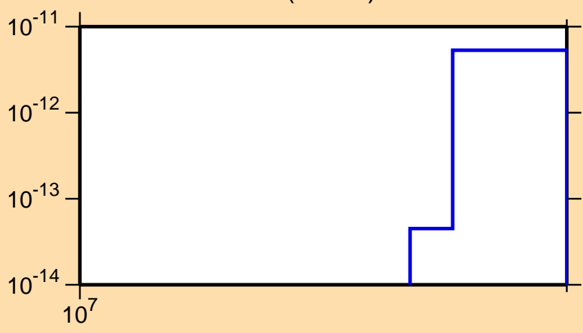
\sigma vs. E for ^{170}\text{W} (mt 34)
