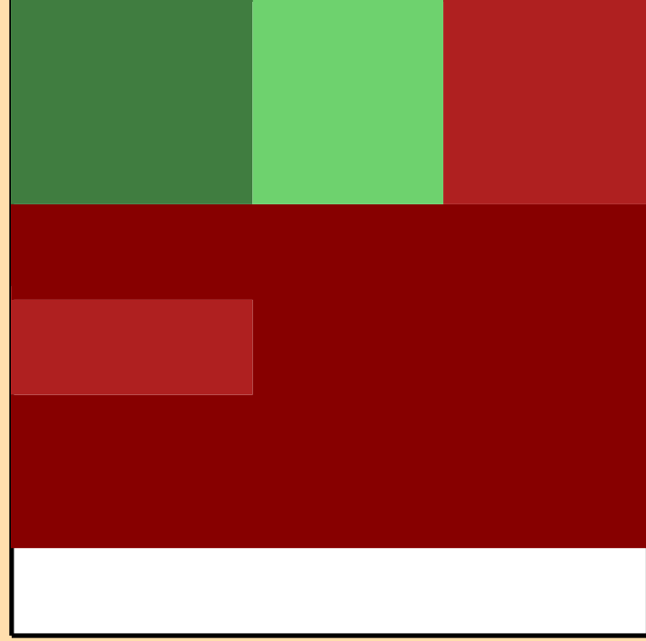
\Delta\sigma/\sigma vs. E for ^{170}\text{W}(n,\text{inel.})
