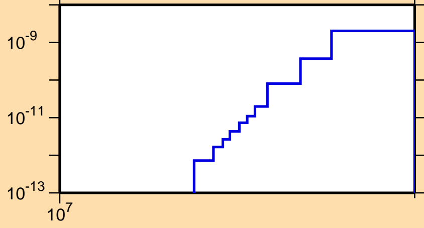
\sigma vs. E for ^{170}\text{W}(\text{mt117})
