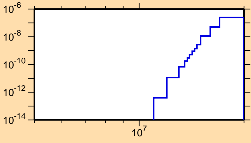
\sigma vs. E for ^{170}\text{W} (mt 45)
