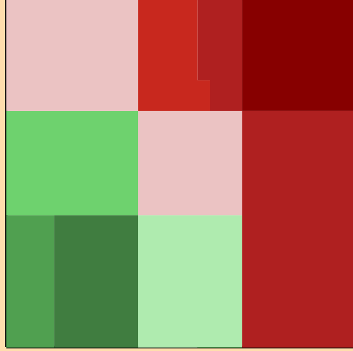
\Delta\sigma/\sigma vs. E for ^{170}\text{W}(n,2n)
