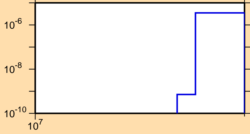
\sigma vs. E for ^{170}\text{W}(n,2np)
