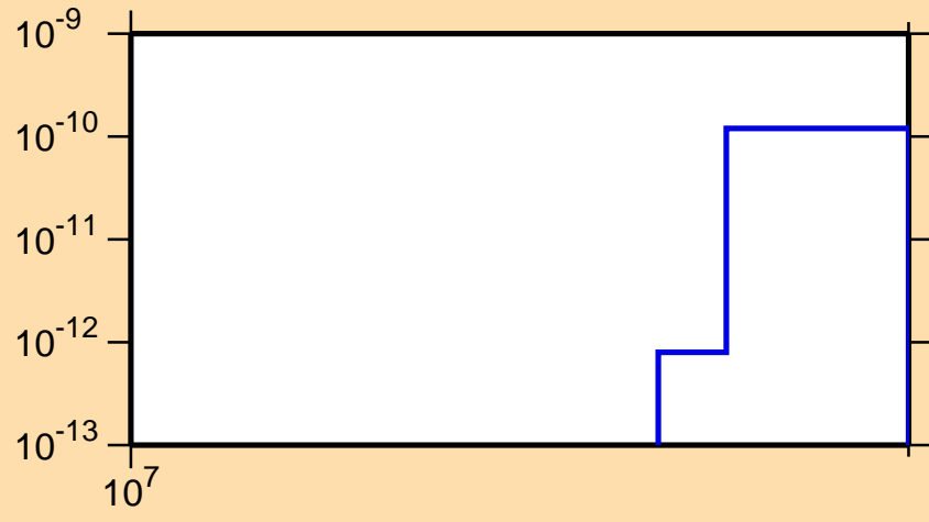
\sigma vs. E for ^{170}\text{W}(n,\text{pt})
