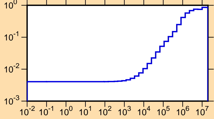
\mu vs. E for ^{170}\text{W}(\text{mt251})
