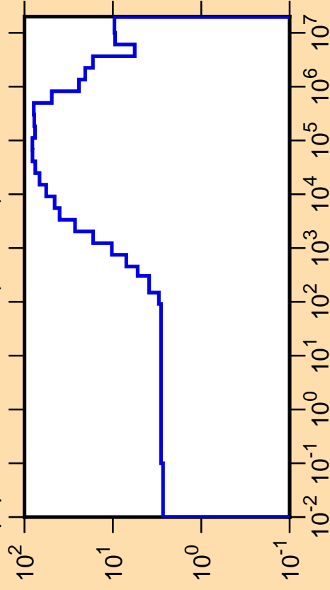
\Delta\mu/\mu vs. E for ^{170}\text{W}(\text{mt251})
