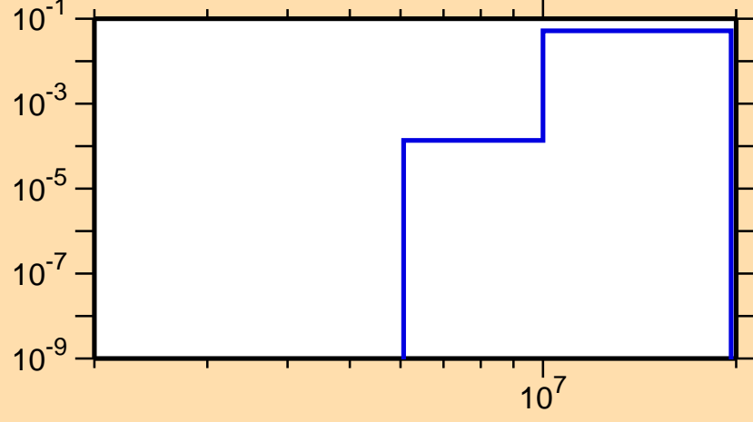
\sigma vs. E for ^{170}\text{W}(n,np)
