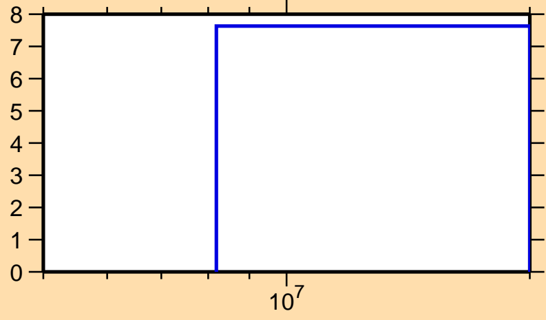
\Delta\sigma/\sigma vs. E for ^{170}\text{W}(n,el.)
