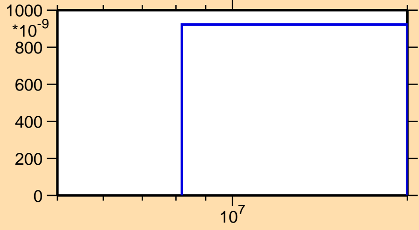
\sigma vs. E for ^{170}\text{W}(n,3n)
