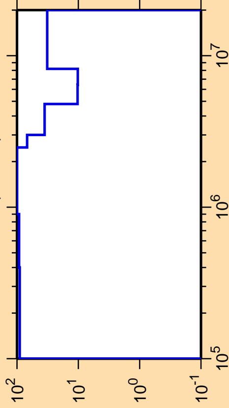
\Delta\sigma/\sigma vs. E for ^{170}\text{W}(n,\text{inel.})
