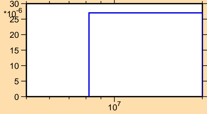
\sigma vs. E for ^{170}\text{W}(n,t)
