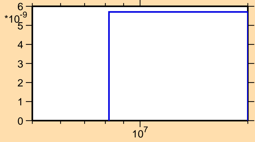
\sigma vs. E for ^{170}\text{W} (mt 45)
