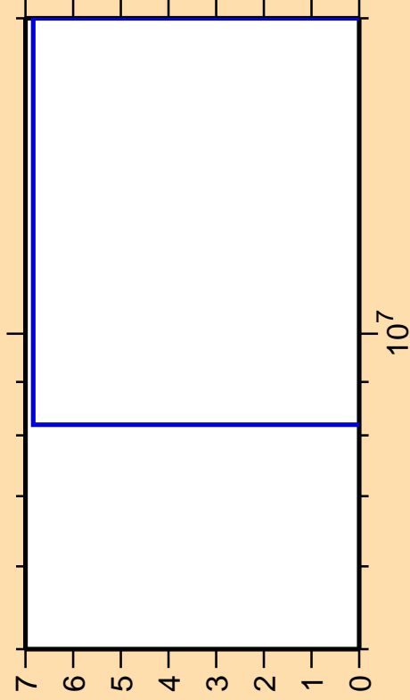
\Delta\sigma/\sigma vs. E for ^{170}\text{W}(n,\text{pt})
