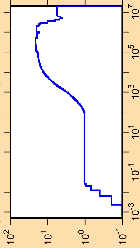
\Delta\mu/\mu vs. E for ^{171}\text{W}(\text{mt251})
