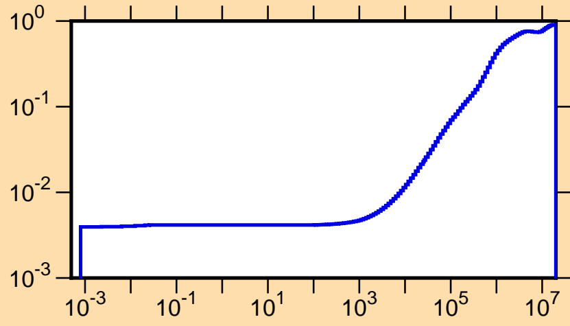
\mu vs. E for ^{171}\text{W}(\text{mt251})
