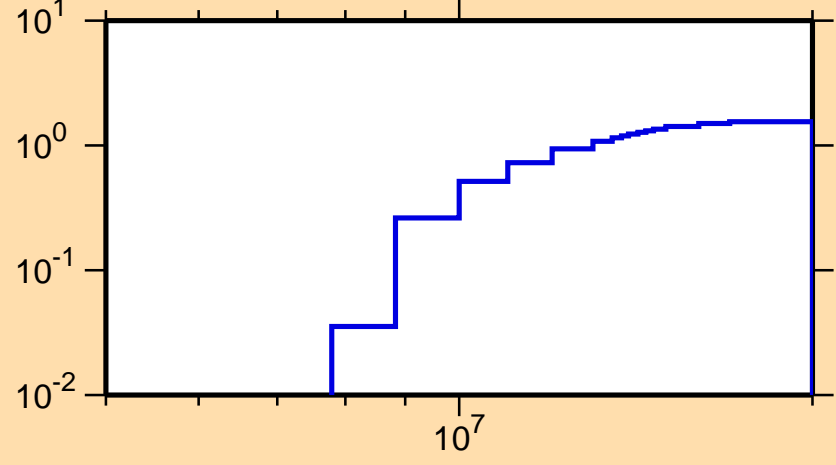
\sigma vs. E for ^{171}\text{W}(n,2n)
