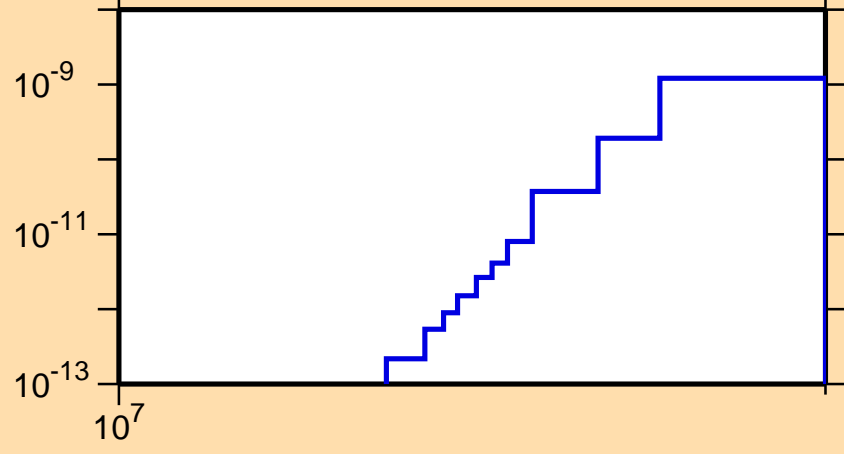
\sigma vs. E for ^{171}\text{W}(\text{mt117})
