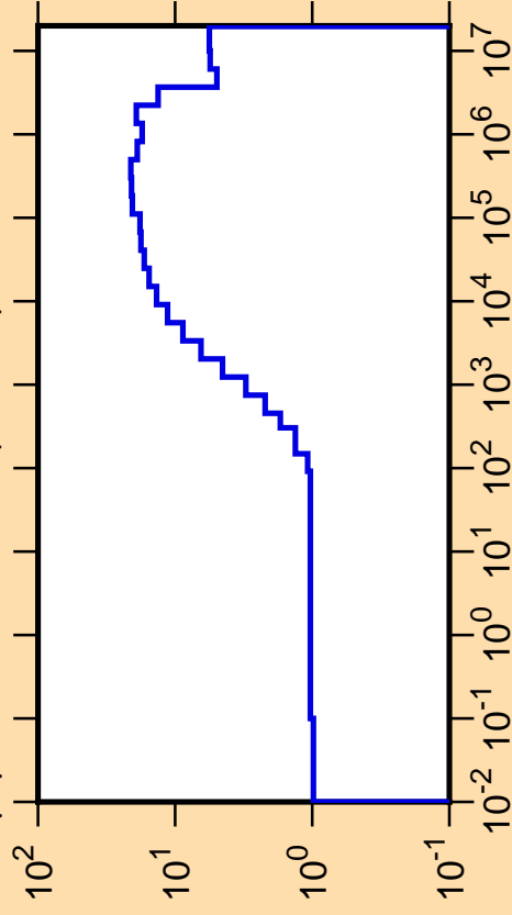
\Delta\mu/\mu vs. E for ^{171}\text{W}(\text{mt251})
