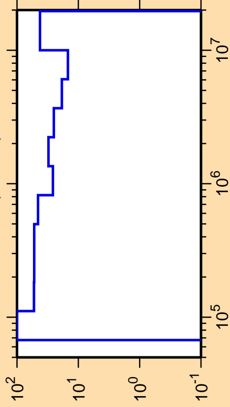
\Delta\sigma/\sigma vs. E for ^{171}\text{W}(n,\text{inel.})
