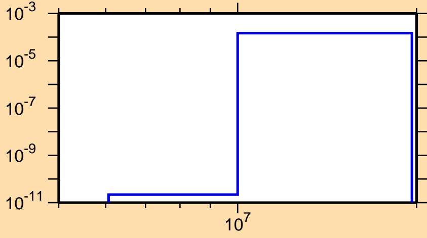
\sigma vs. E for ^{171}\text{W}(n,t)
