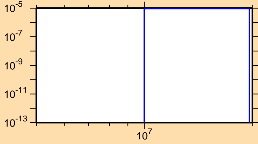
\sigma vs. E for ^{171}\text{W}(n,2n\alpha)
