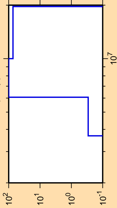
\Delta\sigma/\sigma vs. E for ^{171}\text{W}(n,np)
