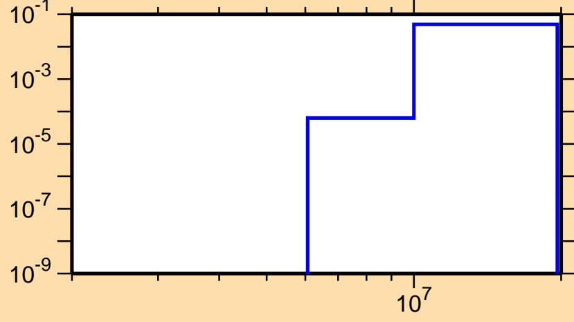
\sigma vs. E for ^{171}\text{W}(n,np)
