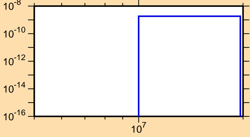
\sigma vs. E for ^{171}\text{W} (mt 45)
