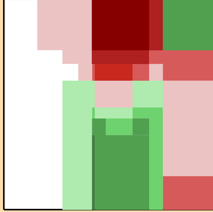
\Delta\sigma/\sigma vs. E for ^{171}\text{W}(n,n\text{cont.})
