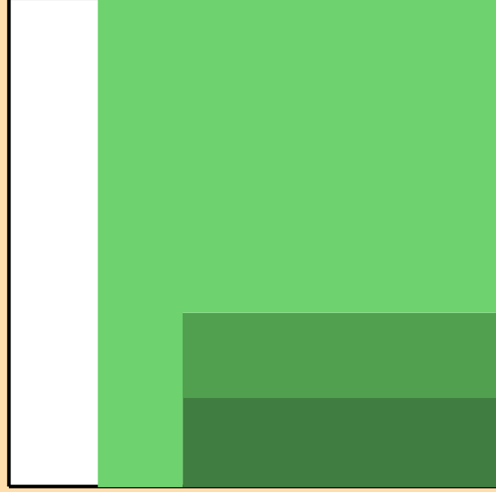
\Delta\sigma/\sigma vs. E for ^{171}\text{W}(n,2n)
