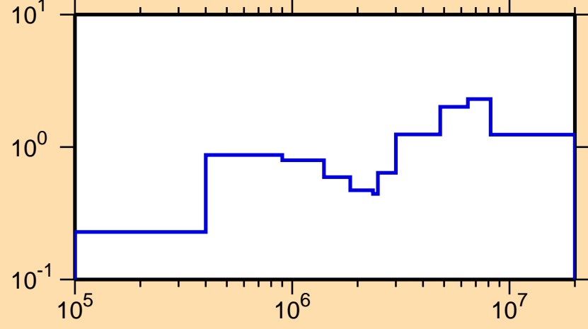
\sigma vs. E for ^{171}\text{W}(n,\text{inel.})
