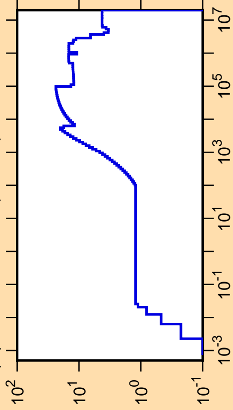
\Delta\mu/\mu vs. E for ^{172}\text{W}(\text{mt251})
