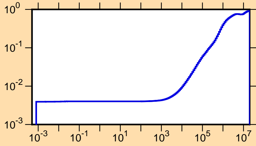
\mu vs. E for ^{172}\text{W}(\text{mt251})
