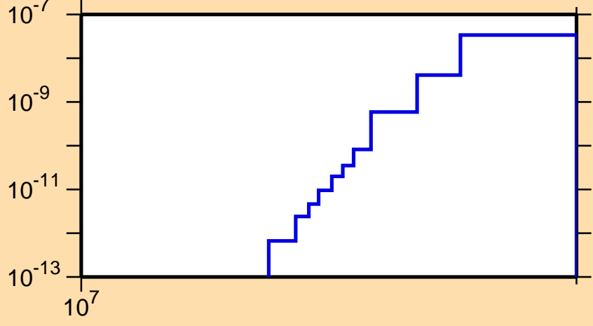
\sigma vs. E for ^{172}\text{W}(n,pd)
