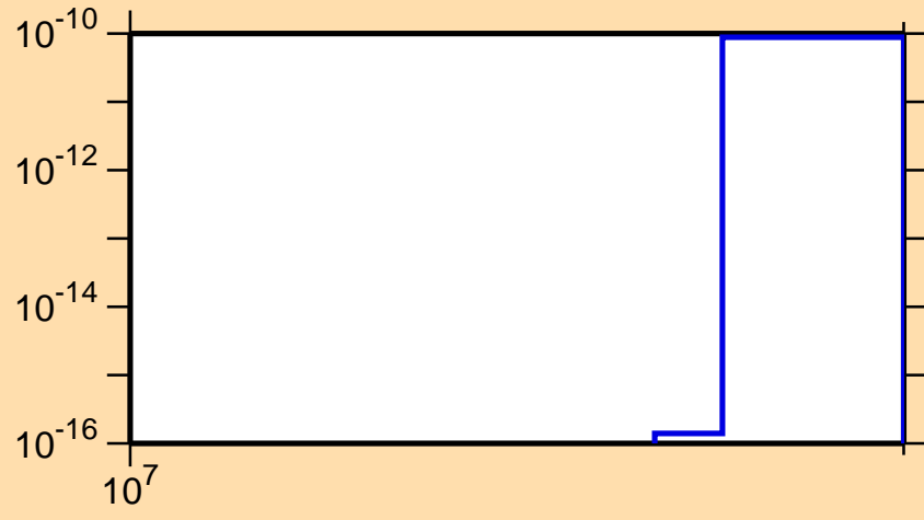
\sigma vs. E for ^{172}\text{W}(n,nt)
