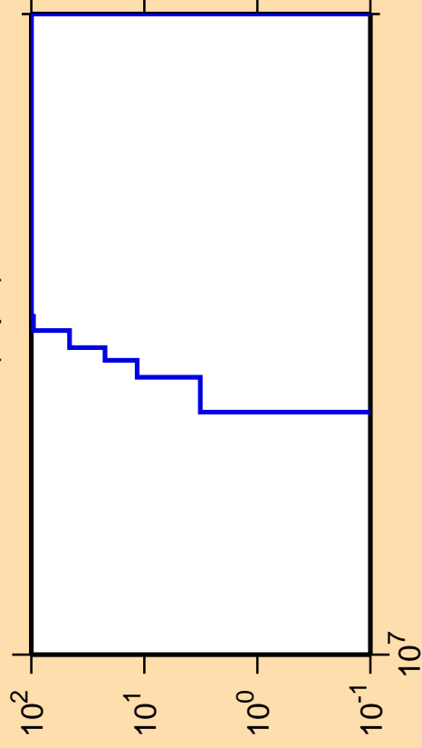
\Delta\sigma/\sigma vs. E for ^{172}\text{W}(n,pd)
