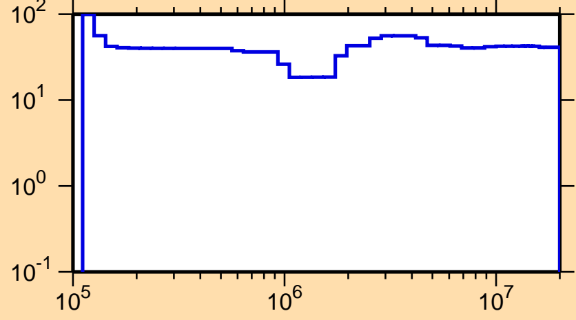
\Delta\sigma/\sigma vs. E for ^{172}\text{W}(n,n_1)
