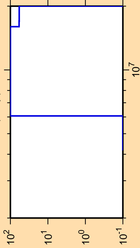
\Delta\sigma/\sigma vs. E for ^{172}\text{W}(n,np)
