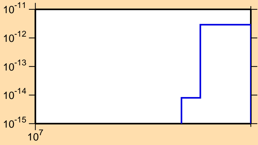
\sigma vs. E for ^{172}\text{W} (mt 34)
