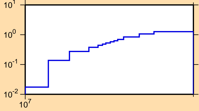
\sigma vs. E for ^{172}\text{W}(n,2n)
