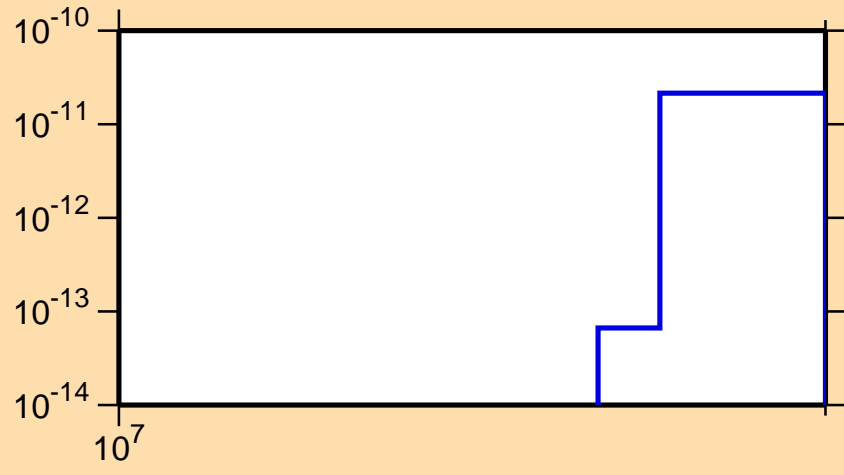
\sigma vs. E for ^{172}\text{W}(n,\text{pt})
