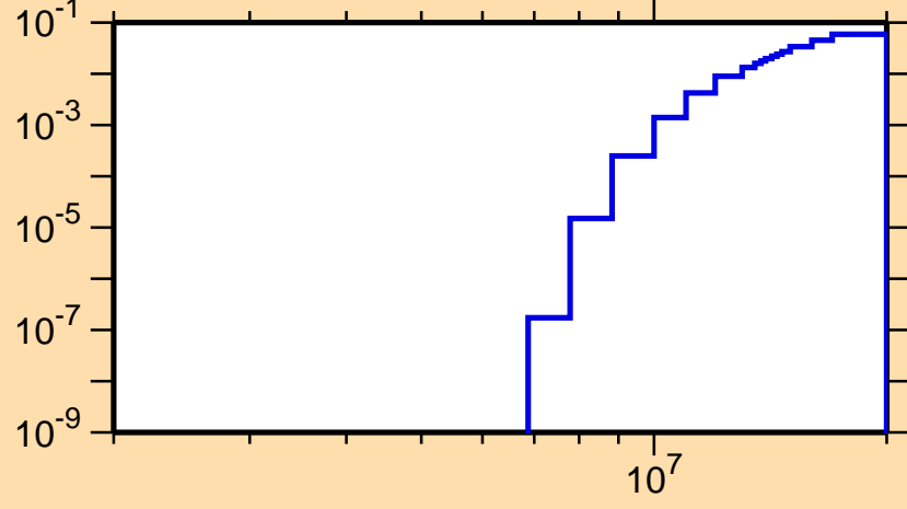
\sigma vs. E for ^{172}\text{W}(n,np)
