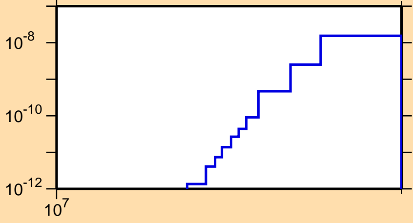
\sigma vs. E for ^{172}\text{W} (mt 45)
