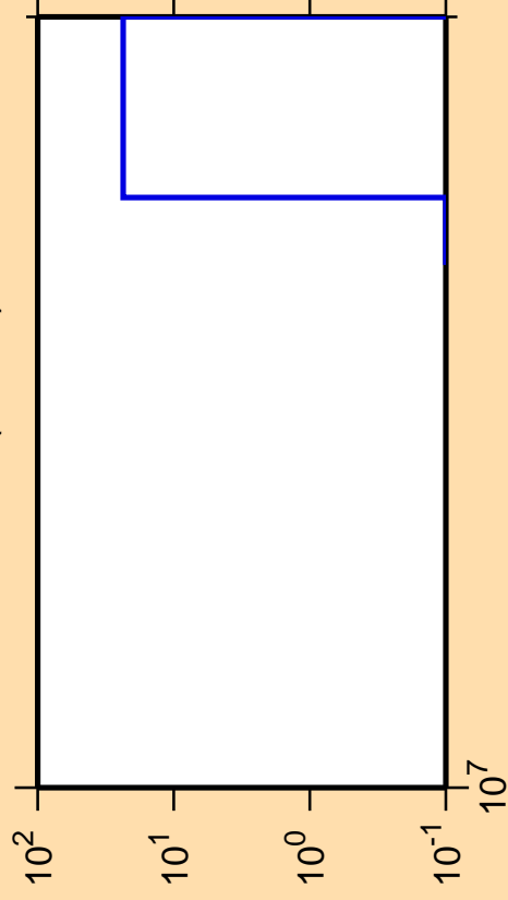
\Delta\sigma/\sigma vs. E for ^{172}\text{W} (mt 34)
