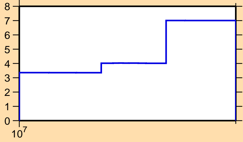
\Delta\sigma/\sigma vs. E for ^{172}\text{W}(n,el.)
