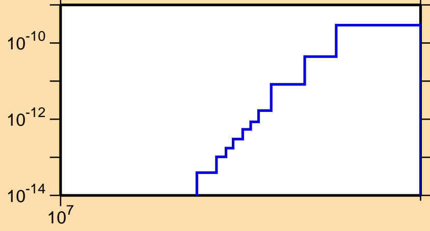
\sigma vs. E for ^{172}\text{W}(\text{mt117})
