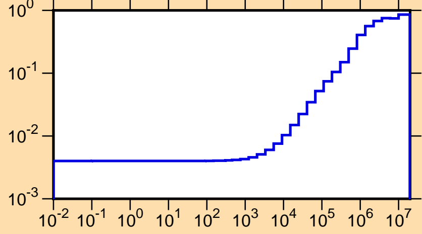
\mu vs. E for ^{172}\text{W}(\text{mt251})
