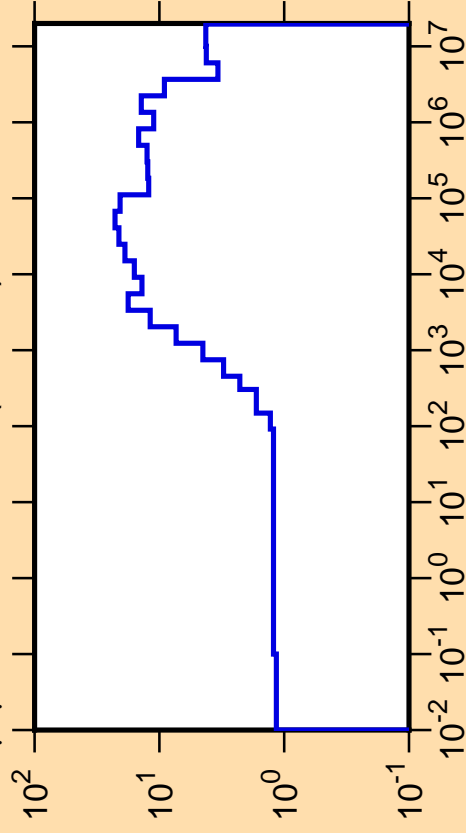
\Delta\mu/\mu vs. E for ^{172}\text{W}(\text{mt251})
