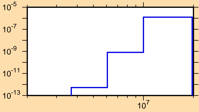
\sigma vs. E for ^{172}\text{W}(n,p\alpha)
