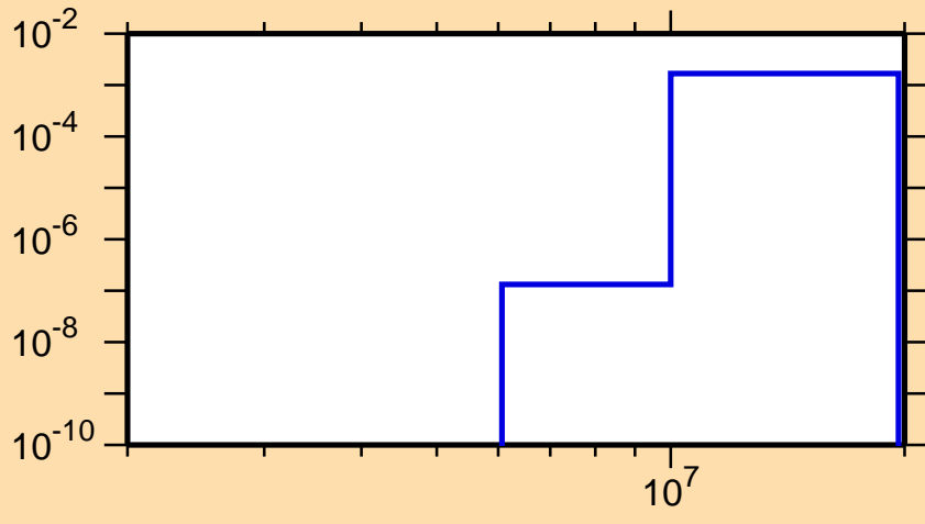
\sigma vs. E for ^{172}\text{W}(n,d)
