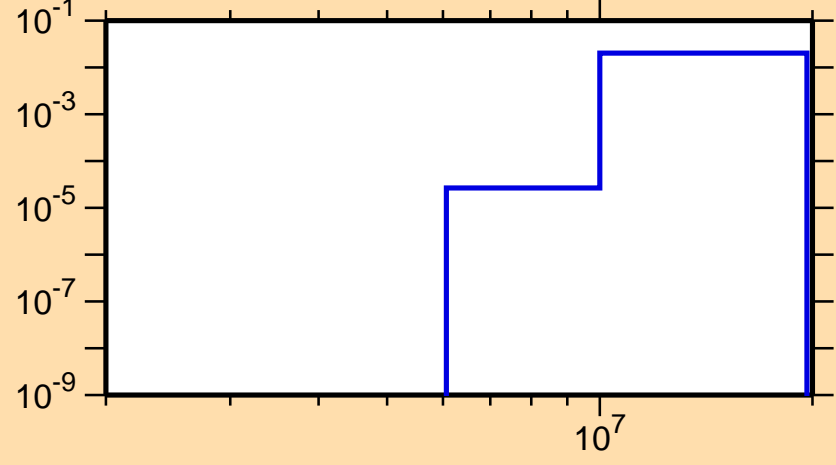
\sigma vs. E for ^{172}\text{W}(n,np)
