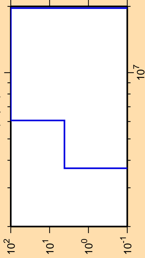
\Delta\sigma/\sigma vs. E for ^{172}\text{W}(n,p\alpha)
