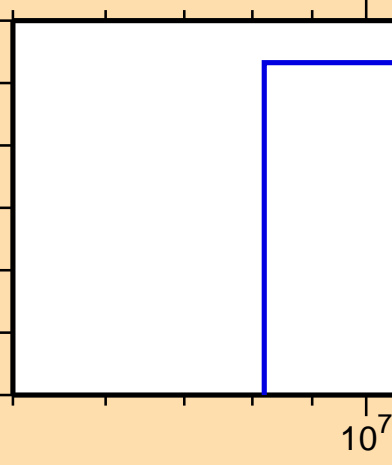
\sigma vs. E for ^{172}\text{W}(\text{mt117})
