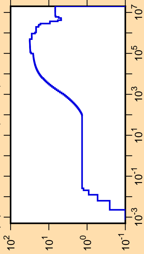
\Delta\mu/\mu vs. E for ^{173}\text{W}(\text{mt251})
