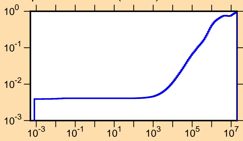
\mu vs. E for ^{173}\text{W}(\text{mt251})
