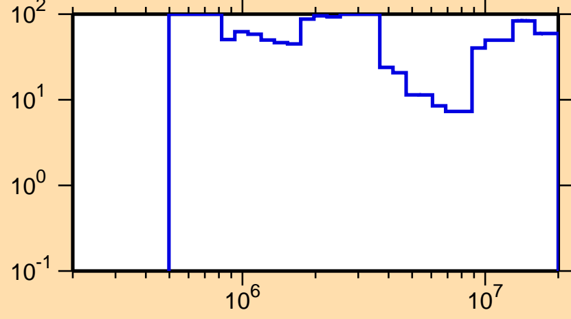
\Delta\sigma/\sigma vs. E for ^{173}\text{W}(n,n\text{cont.})
