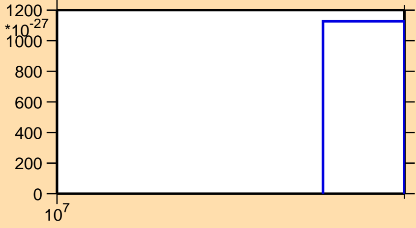
\sigma vs. E for ^{173}\text{W} (mt 11)
