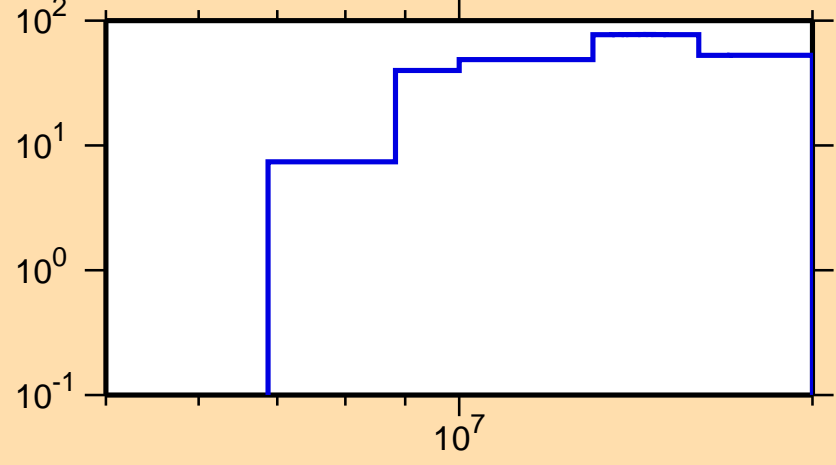
\Delta\sigma/\sigma vs. E for ^{173}\text{W}(n,\text{inel.})
