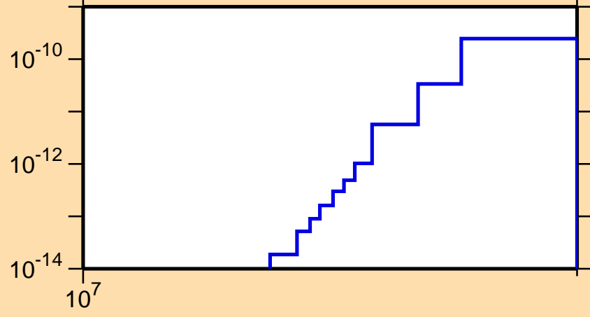
\sigma vs. E for ^{173}\text{W}(\text{mt117})
