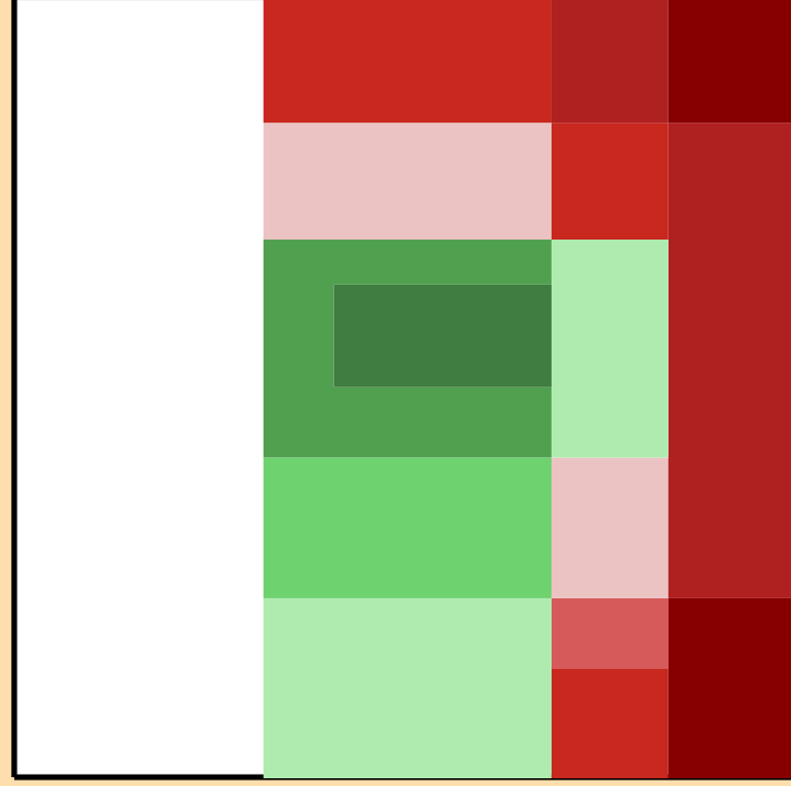
\Delta\sigma/\sigma vs. E for ^{173}\text{W}(n,2n)
