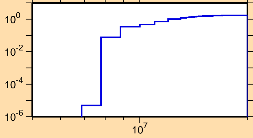
\sigma vs. E for ^{173}\text{W}(n,2n)
